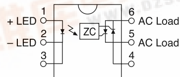
PM1204 Pinout
