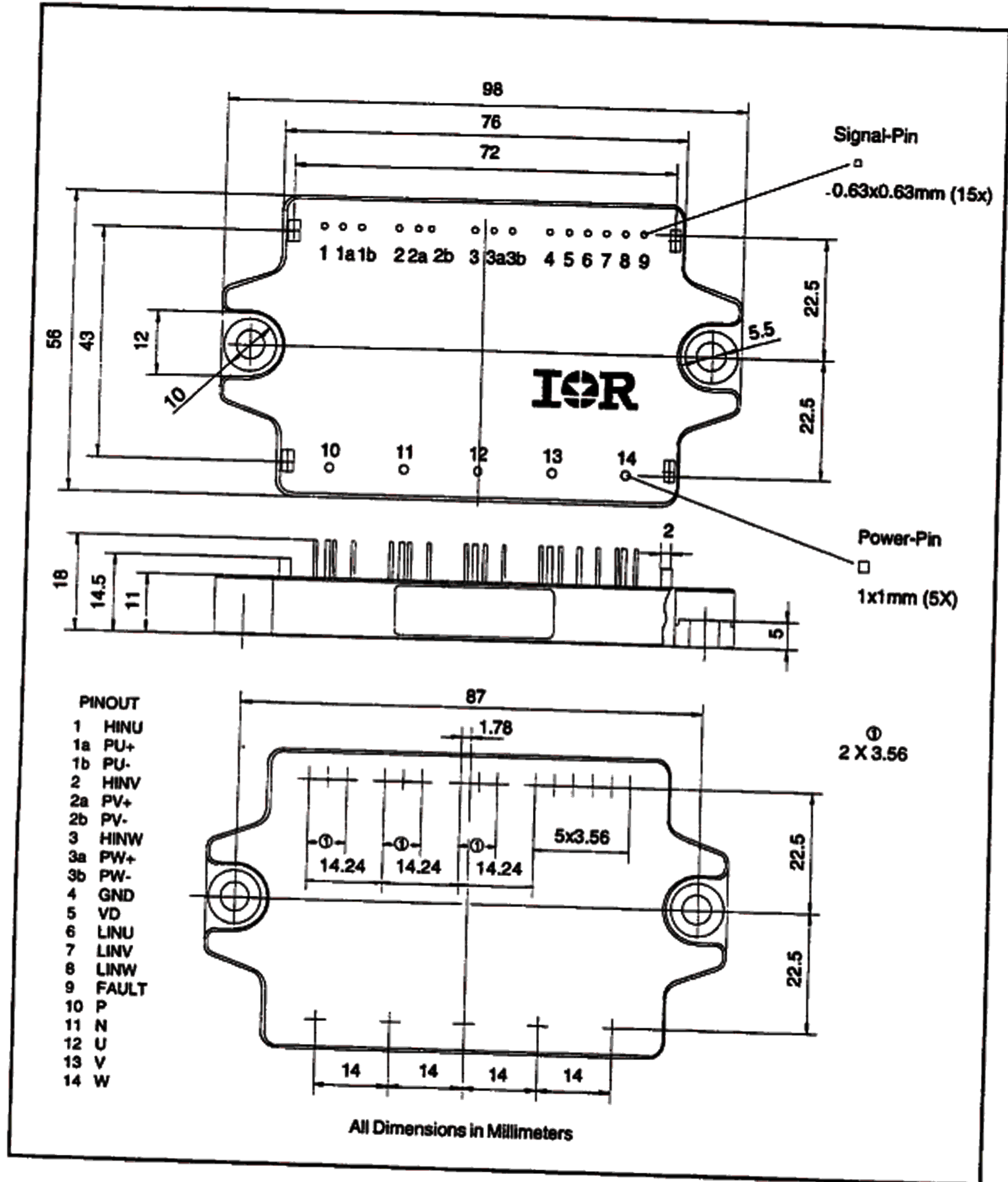
Fig. 7 - Package Outline
