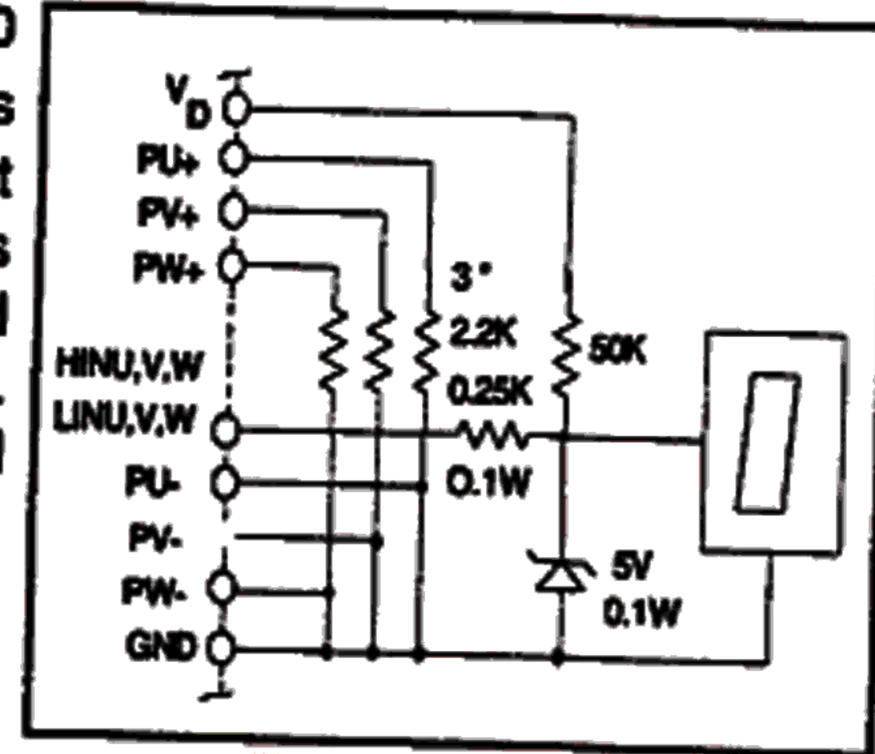
Figure 8: Input Stage
