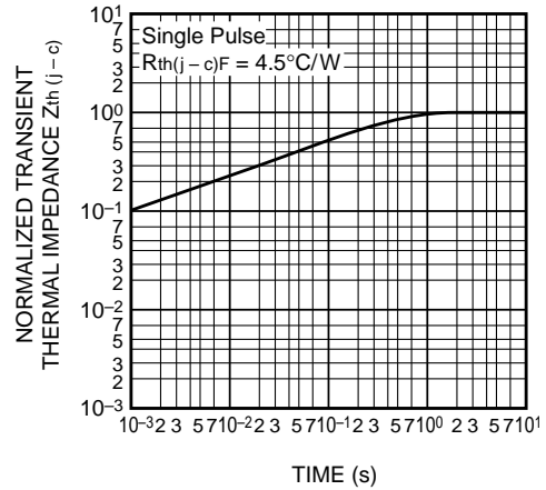
TRANSIENT THERMAL IMPEDANCE CHARACTERISTICS (FWDi per 1 element)
