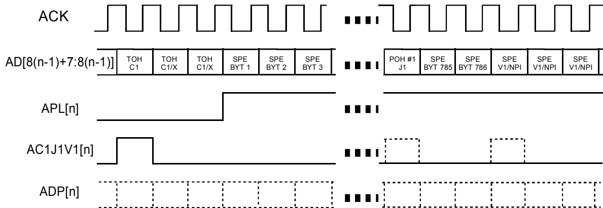
Figure 42 STS-3c (STM-1/AU-4) 19.44 MHz Byte Add Bus Timing
