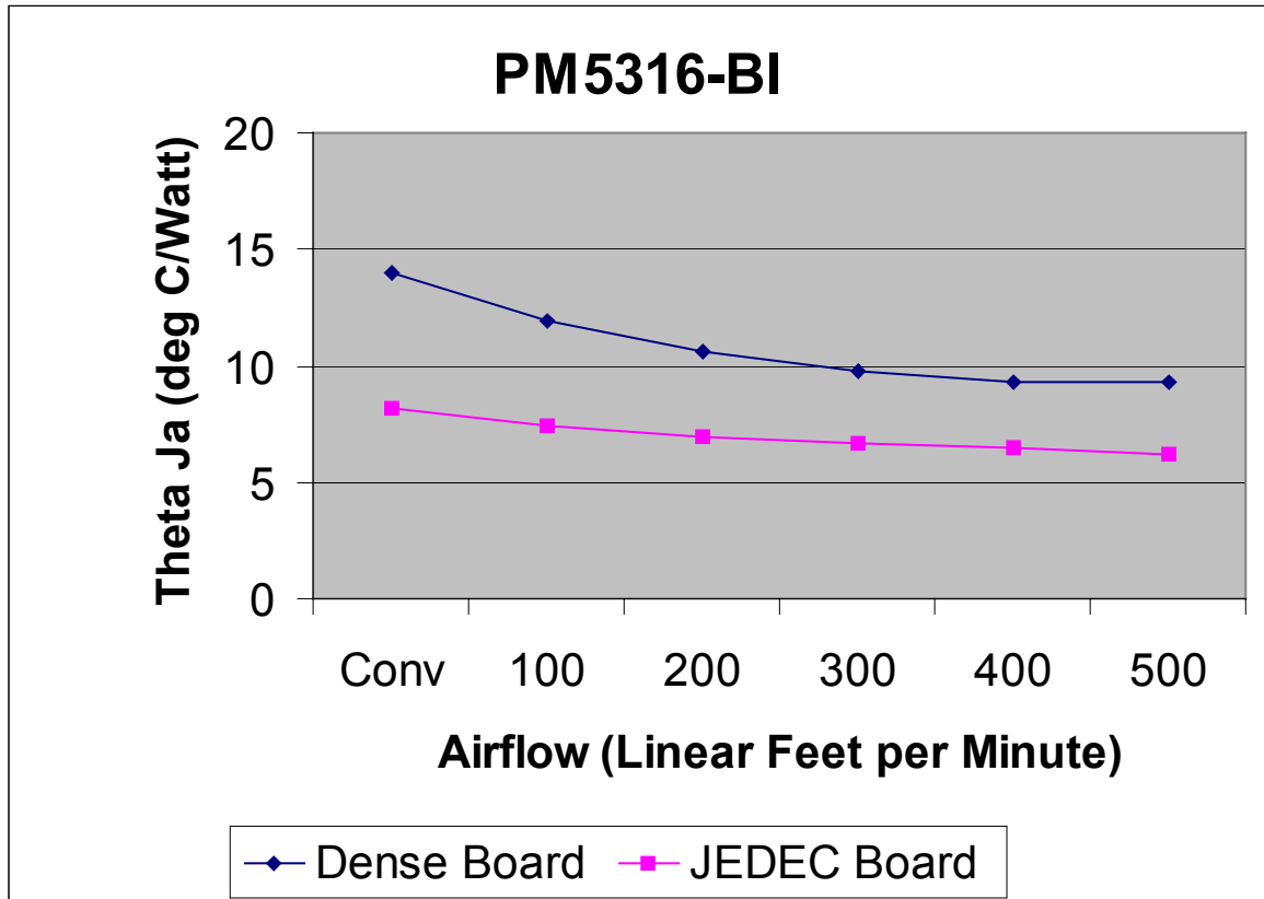
Figure 67 Theta Ja vs. Airflow Plot
