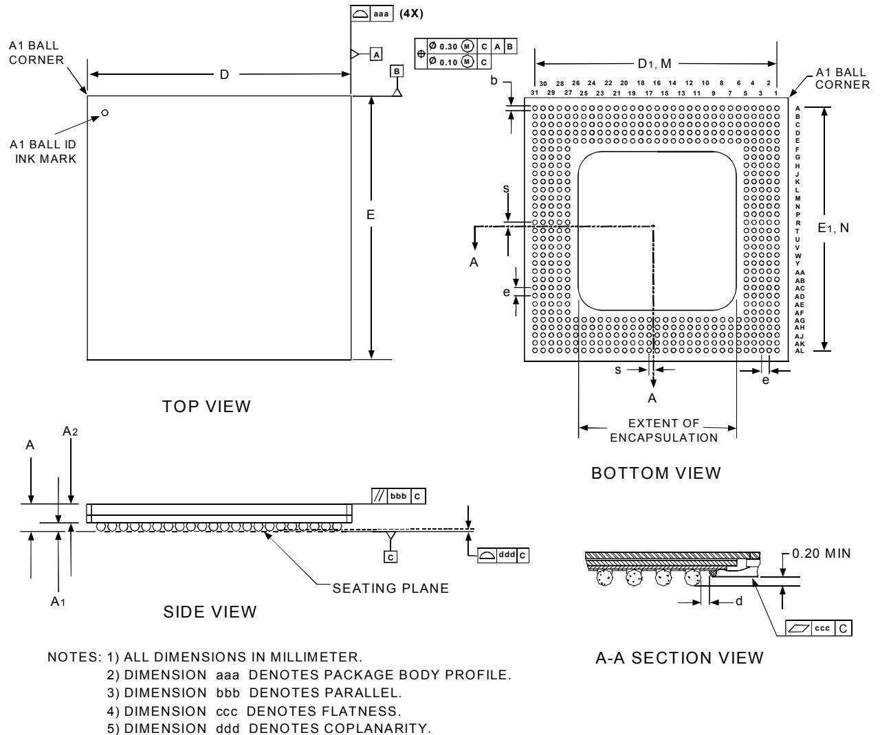
Figure 68 Mechanical Drawing 520 Pin Super Ball Grid Array (SBGA)
