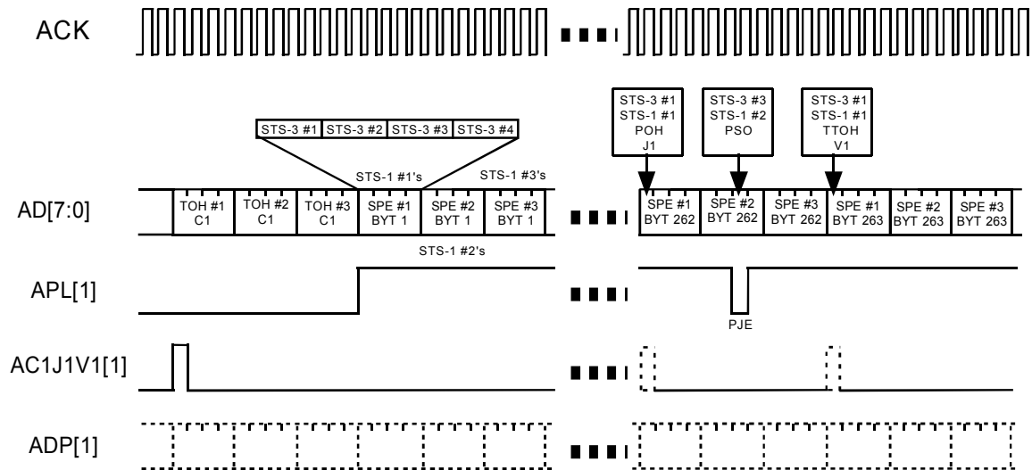
Figure 44 STS-12 (STM-12/AU-3) 77.76 MHz Byte Add Bus Timing
