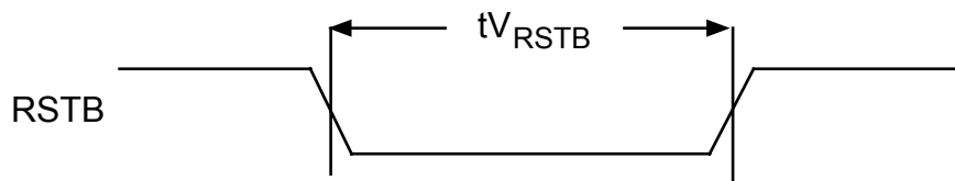
Figure 52 - RSTB Timing Diagram
