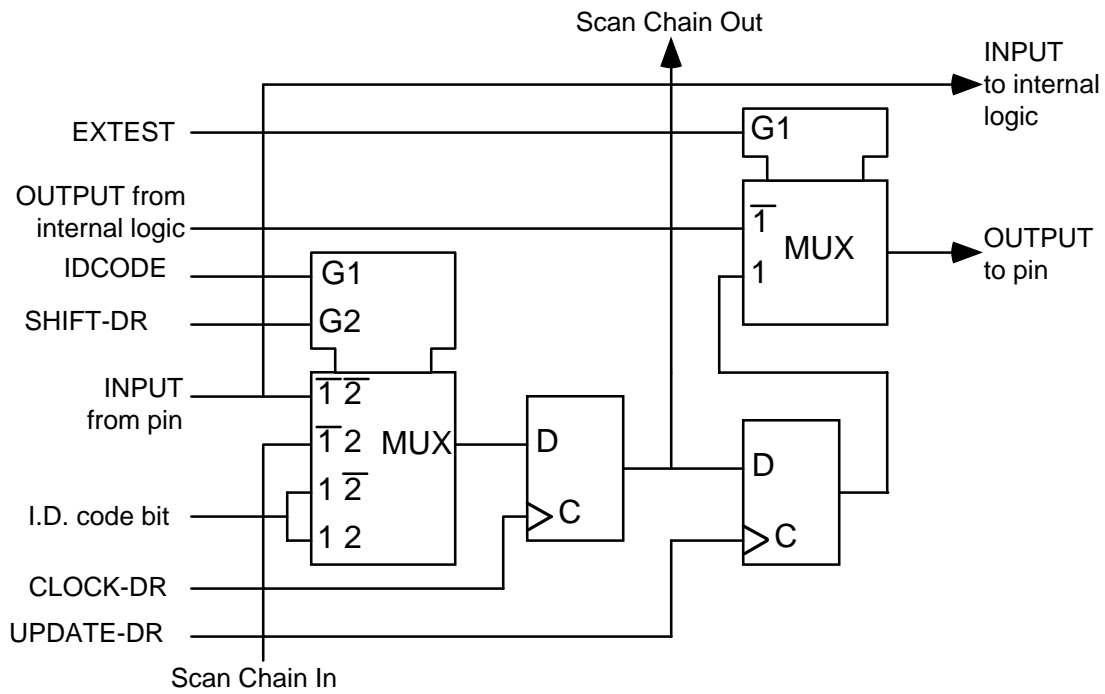
Figure 21 - Bidirectional Cell (IO_CELL)
