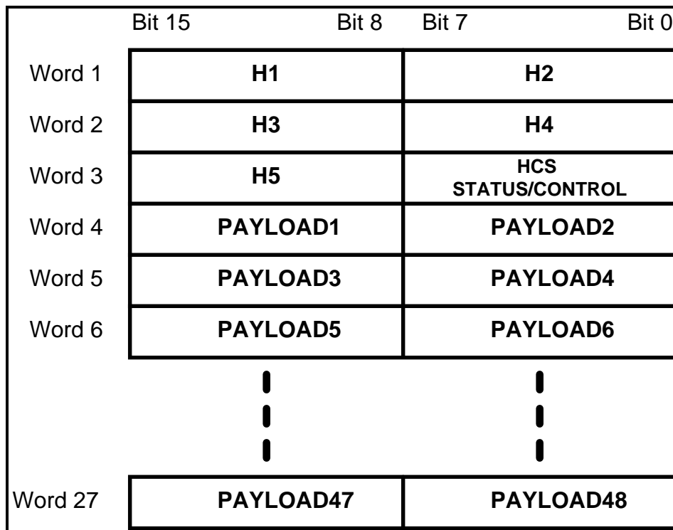
Figure 15 - 16-bit Wide, 27 Word Structure
