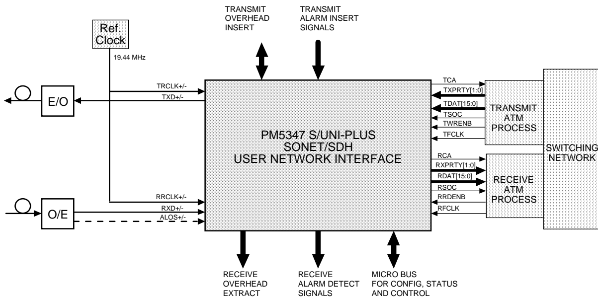
Figure 1 - Typical STS-3c ATM Switch Port Interface
