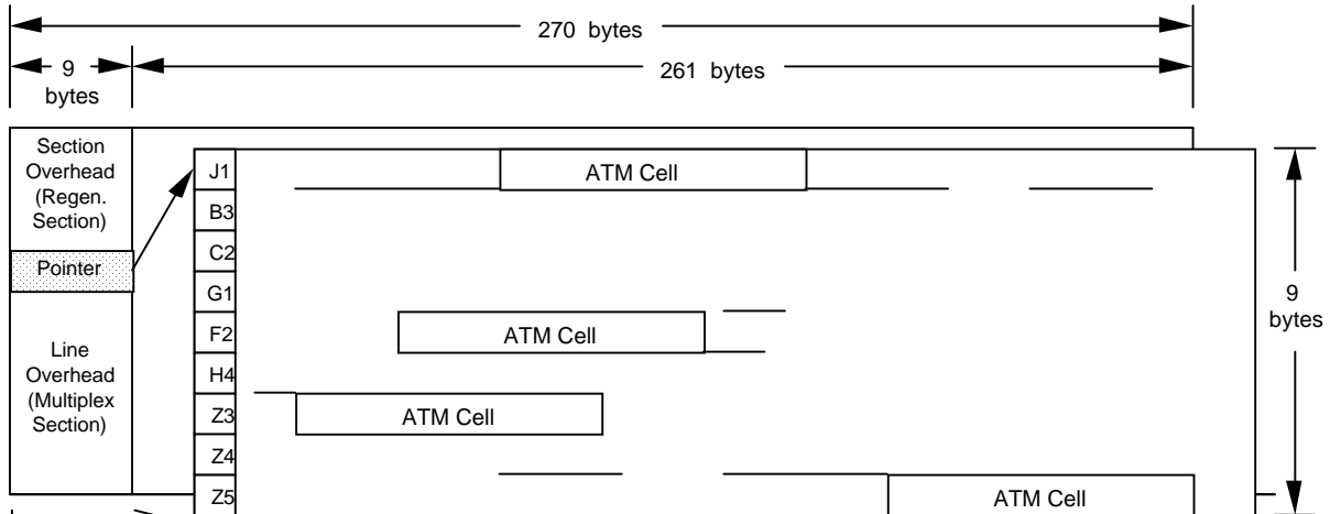
STS-3c Transport Overhead STM-1 Section Overhead
