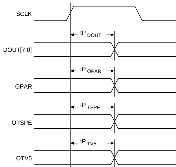
Figure 22 - Output Timing
