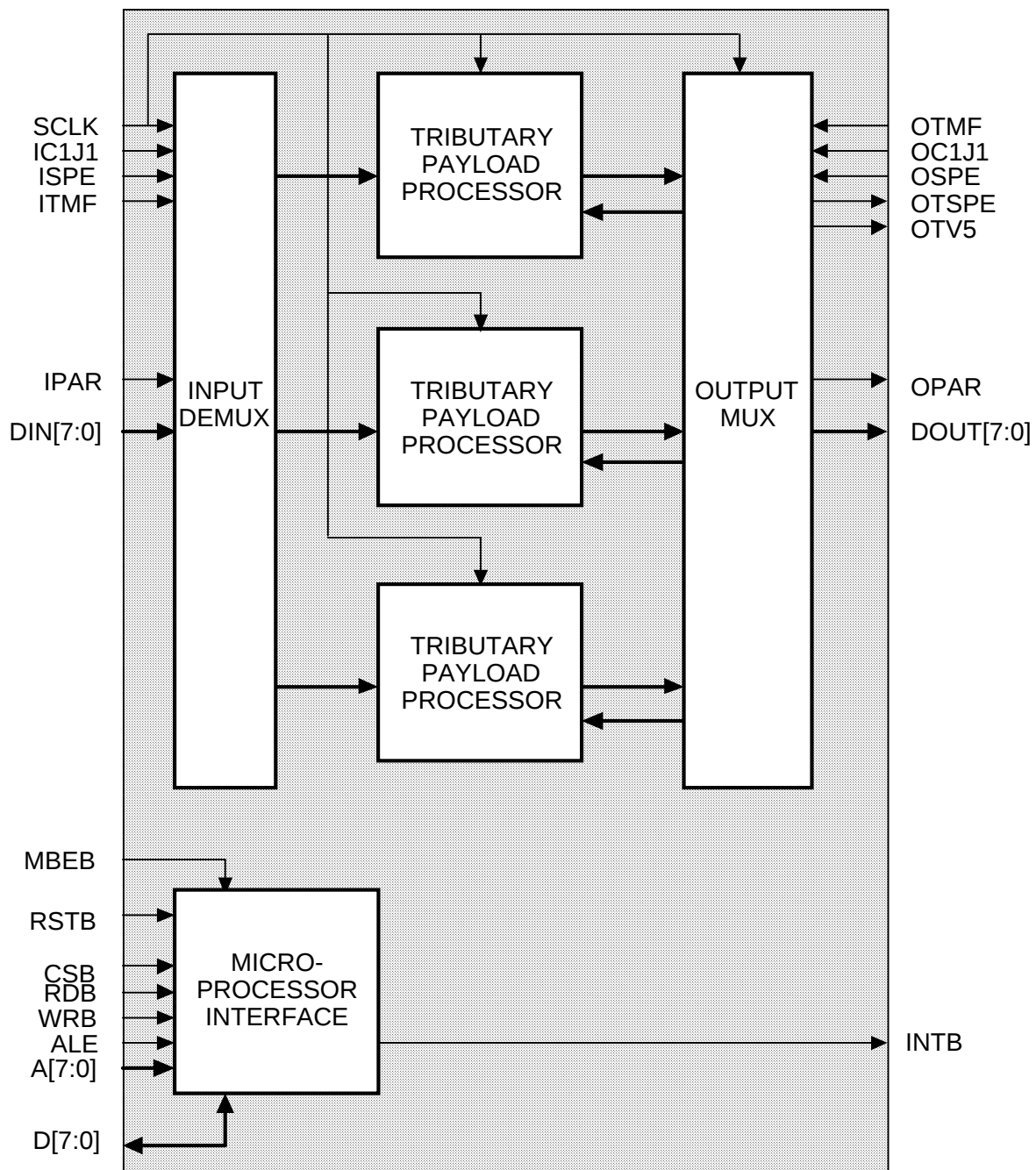
Figure 2 - Overall Device
