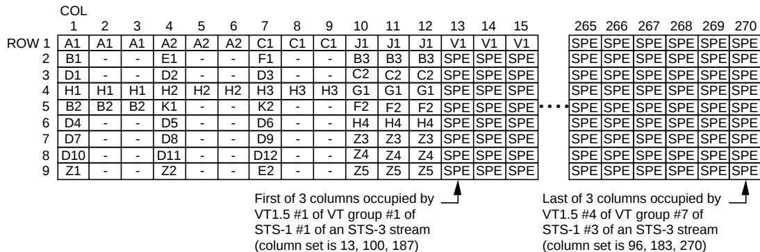
Figure 4 - SONET STS-3 Carrying VT1.5 Within STS-1
