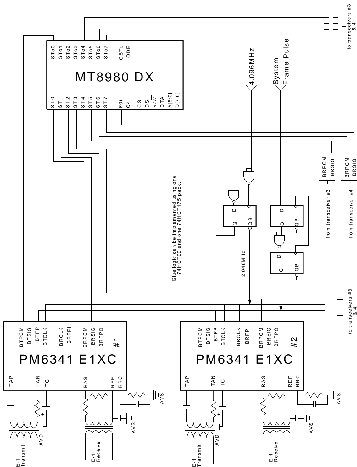
Figure 2 - DS0 Cross-connect
