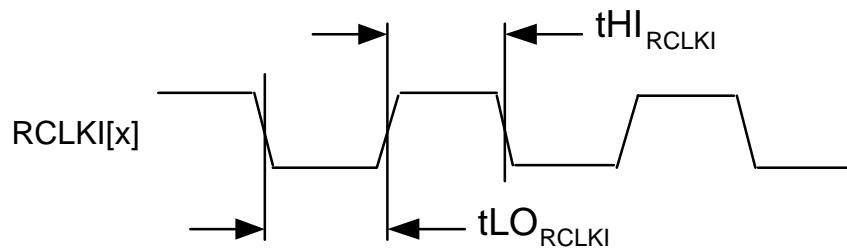
Figure 41 - Digital Receive Interface Input Timing Diagram
