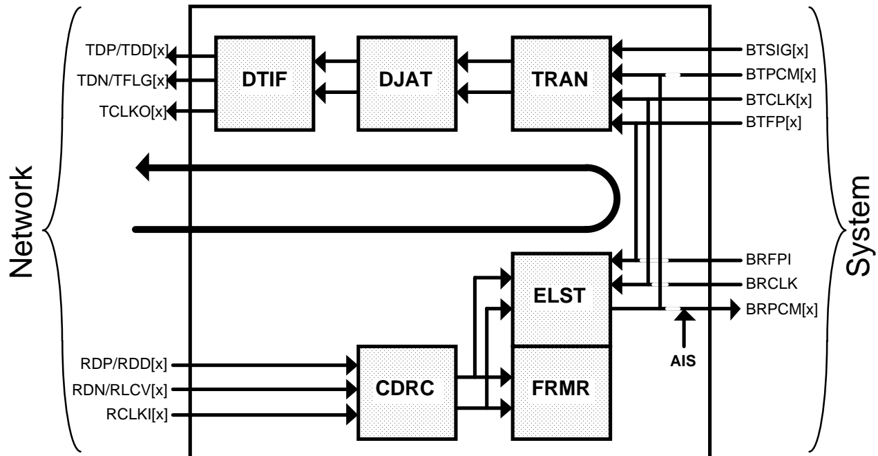
Figure 28 - Payload Loopback
