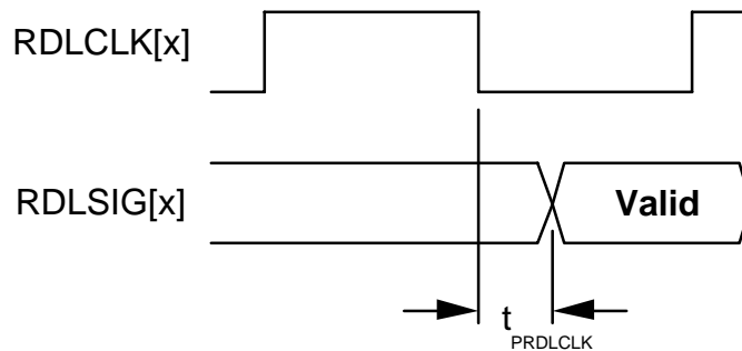
Figure 46 - Receive Data Link Output Timing Diagram
