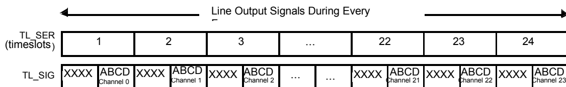
Figure 77 Output of T1 Signaling Bits
