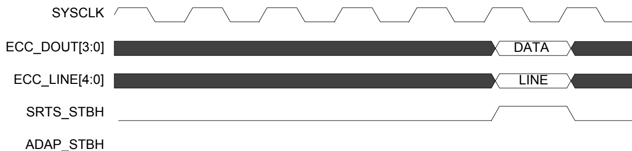
Figure 115 SRTS Data
