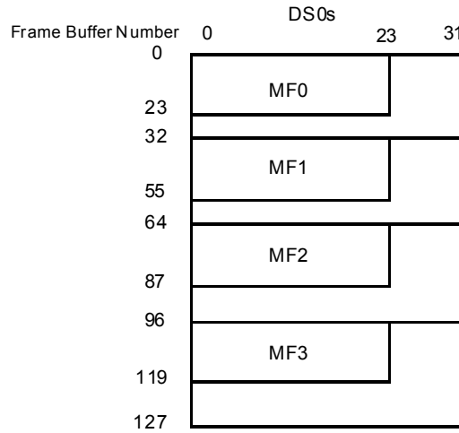
Figure 13 T1 ESF SDF-MF Format of the T_DATA_BUFFER
