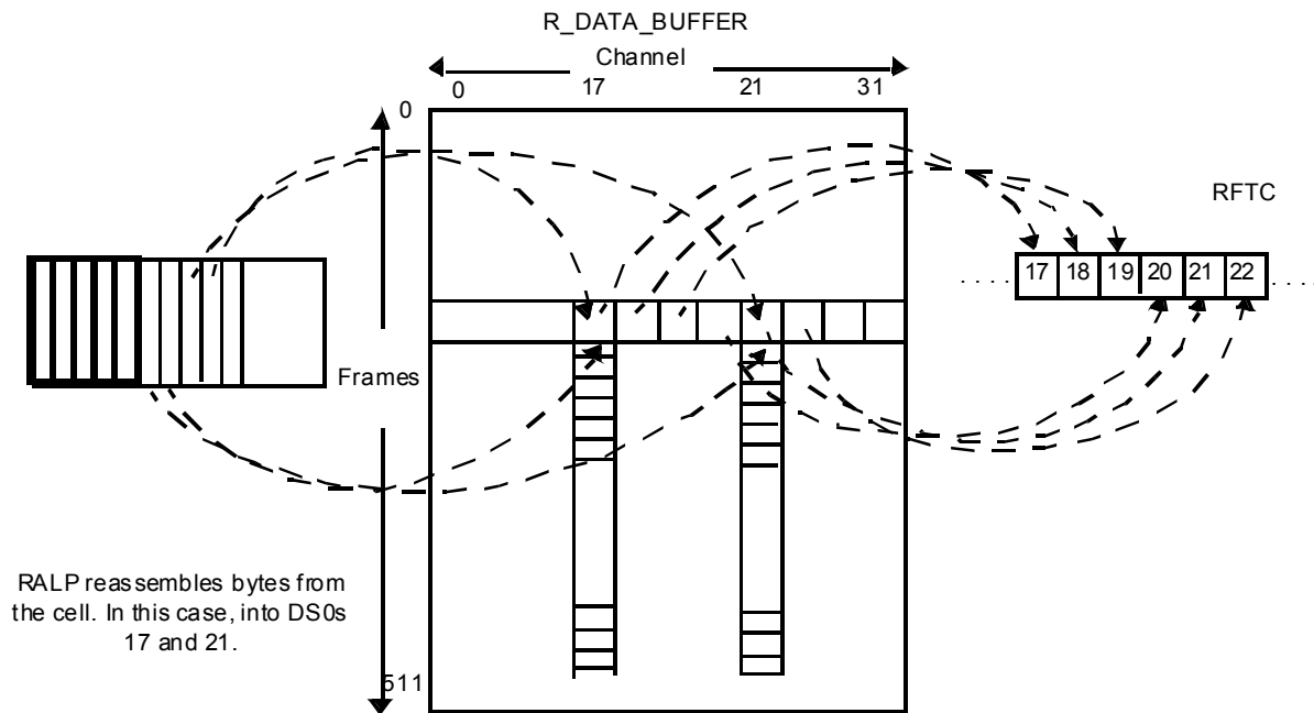
Figure 40 Cell Reception
