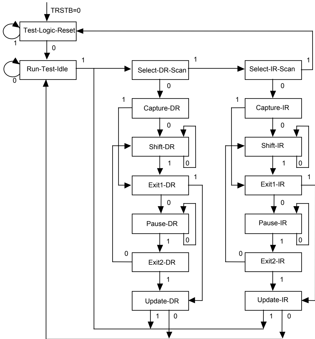
Figure 86 TAP Controller Finite State Machine
