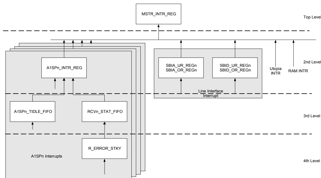
Figure 71 Interrupt Hierarchy
