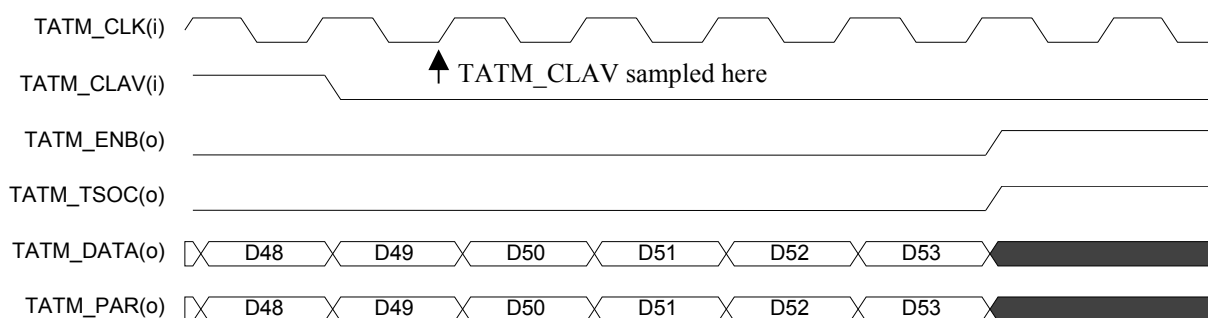
Figure 94 SRC_INTF End-of-Transfer Timing (Utopia 1 ATM Mode)
