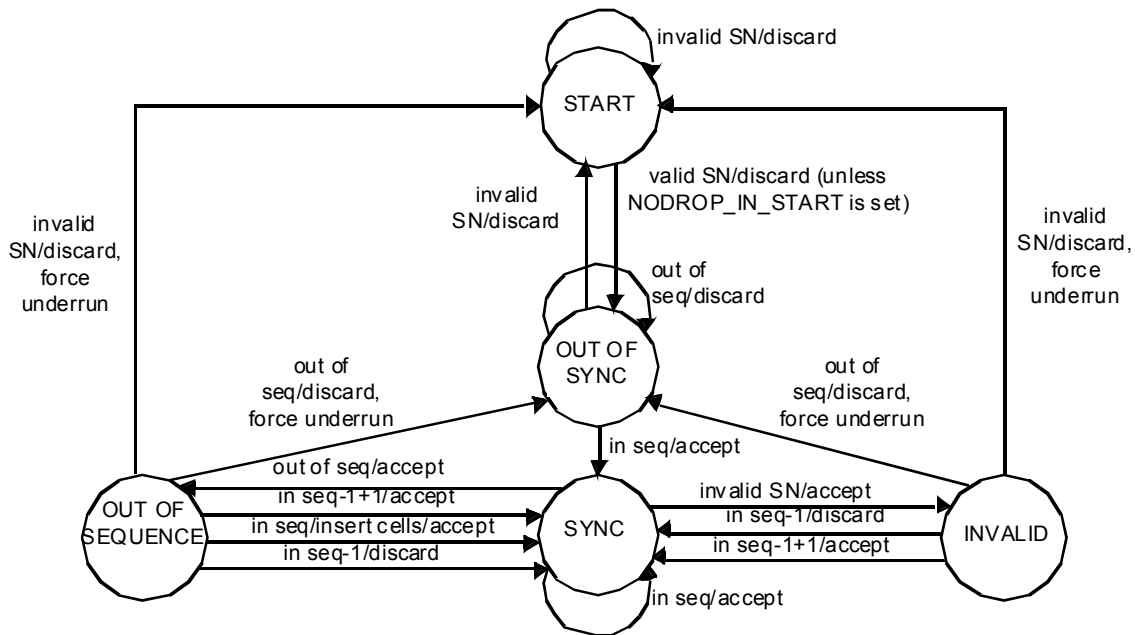
Figure 37 Fast SN Algorithm
