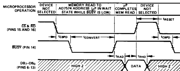
Figure 3. Slow Memory Mode Timing Diagram ( \overline{CS} and \overline{RD} Tied Together)
