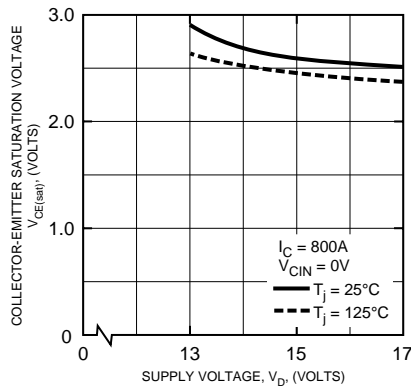
COLLECTOR-EMITTER SATURATON VOLTAGE CHARACTERISTICS (TYPICAL)
