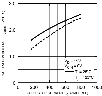
SATURATON VOLTAGE CHARACTERISTICS (TYPICAL)
