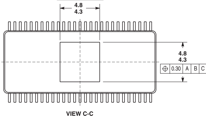
VIEW C-C
