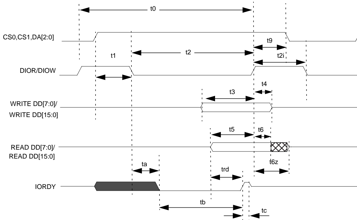
Figure 12: Register Transfer/PIO Data Transfer on IDE
