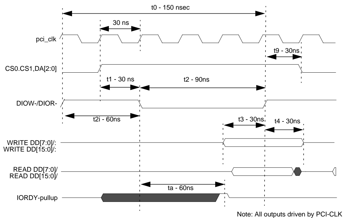
Figure 13: Timings on IDE Bus
