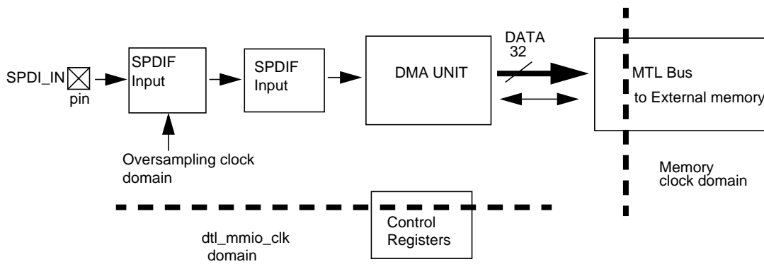
Figure 1: SPDIF Input Block Diagram
