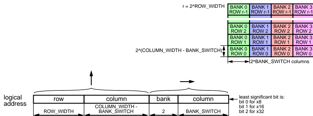
Figure 6: Address Mapping: Interleaved Mode
