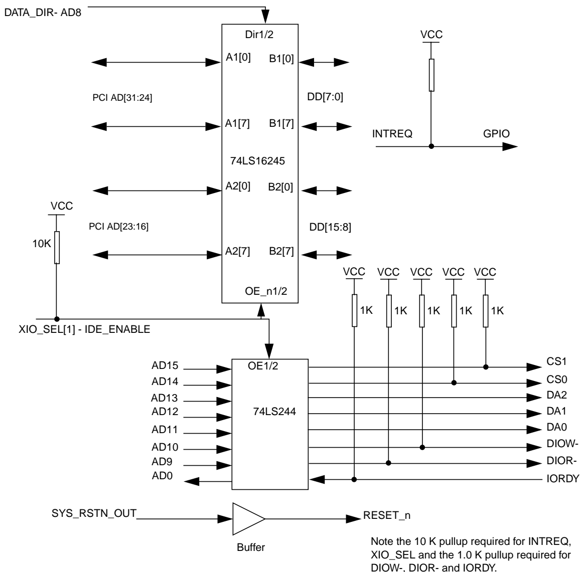
Figure 11: Isolation Translation Logic
