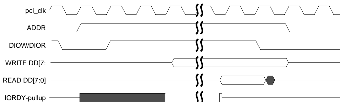
Figure 14: IDE Transaction, Flow Controlled by Device IORDY
