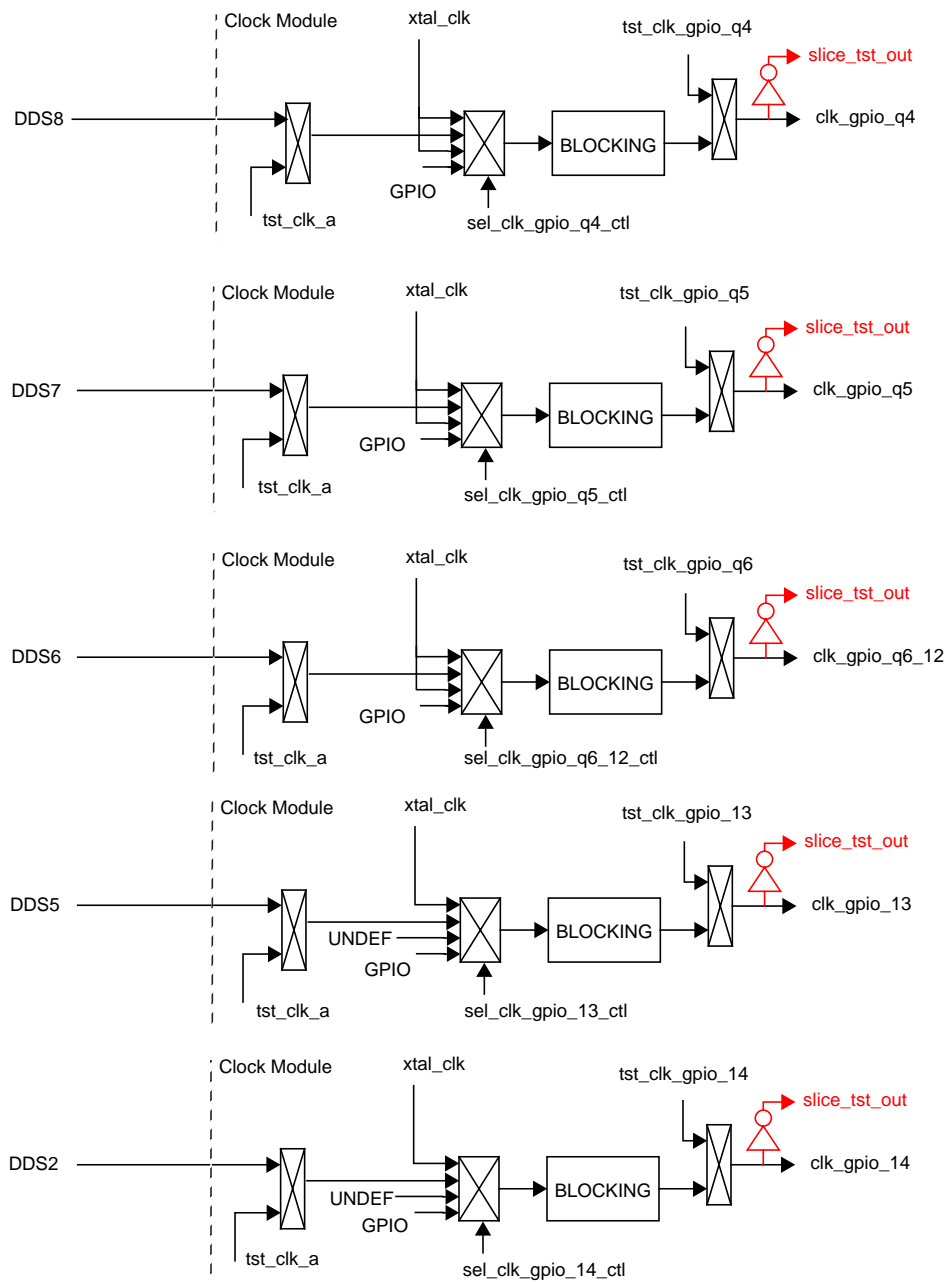
Figure 14: GPIO Clocks
