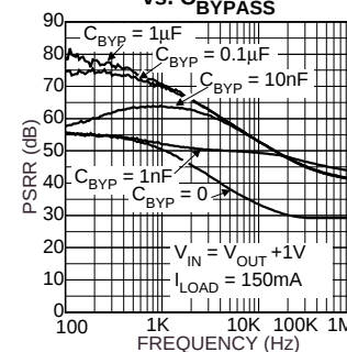
Power Supply Rejection Ratio vs. C_{BYPASS}
