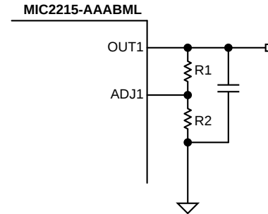
Figure 1. Adjustable Output
