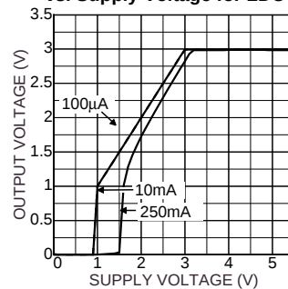
Output Voltage vs. Supply Voltage for LDO 2
