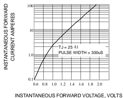
Fig. 4-TYPICAL FORWARD CHARACTERISTIC
