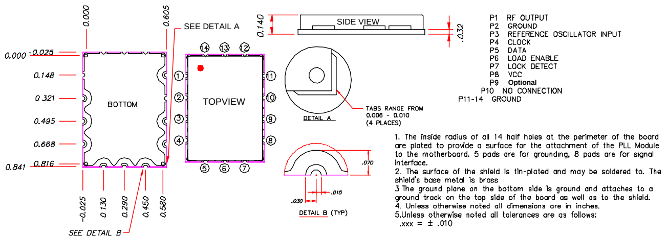
PHYSICAL DIMENSIONS
