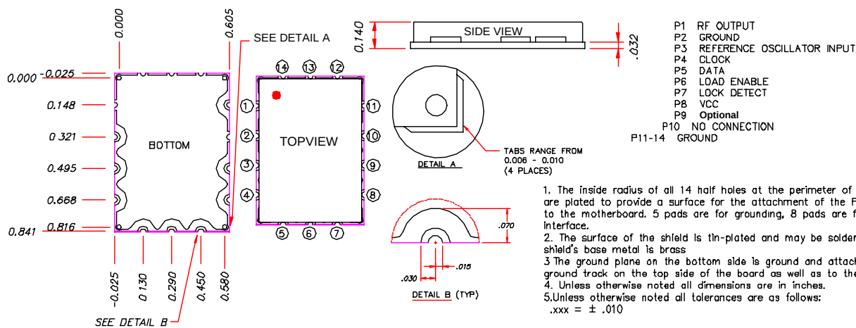
PHYSICAL DIMENSIONS
