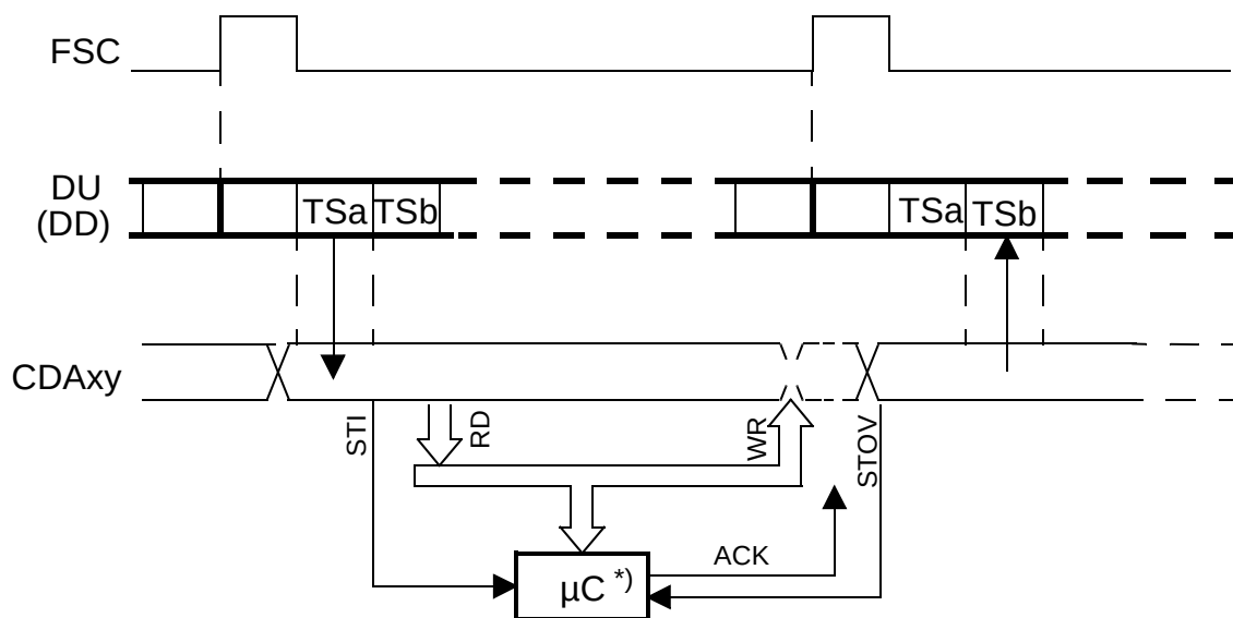
Figure 54 Data Access When Shifting TSa to TSb on DU (DD)
