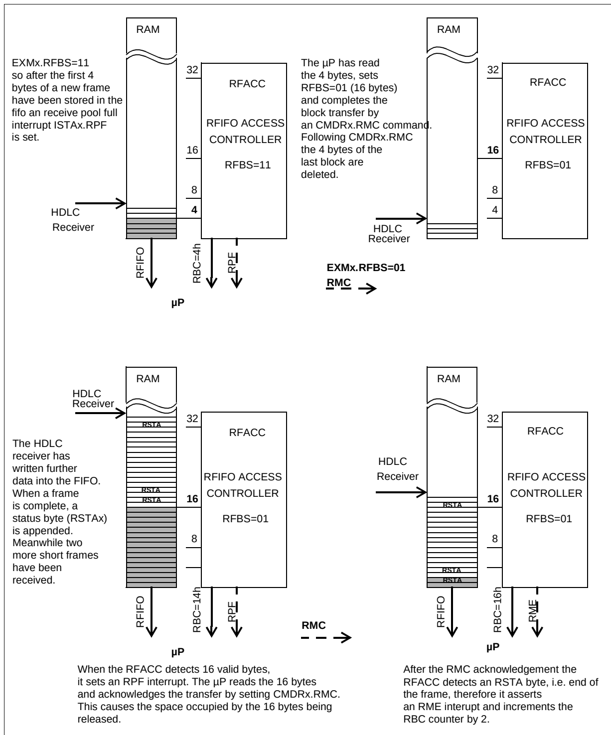
Figure 78 RFIFO Operation
