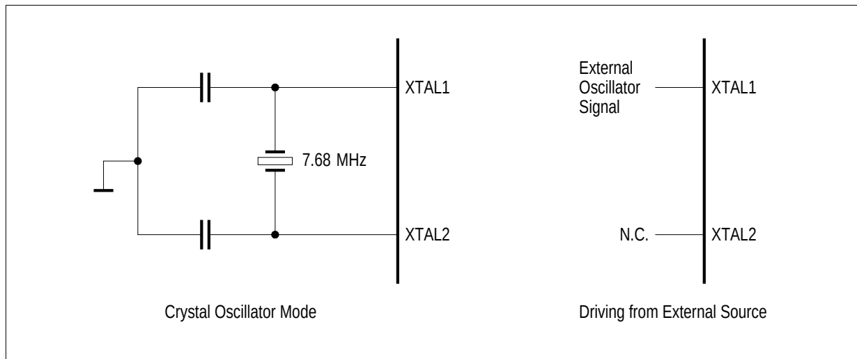
Figure 88 Oscillator Circuits
