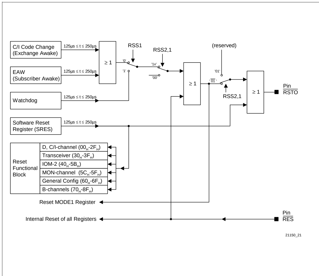
Figure 12 Reset Generation
