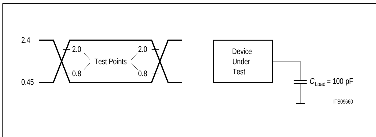
Figure 89 Input/Output Waveform for AC Tests
