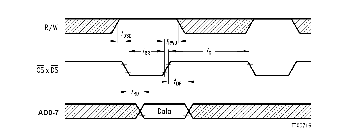
Figure 98 Microprocessor Read Timing
