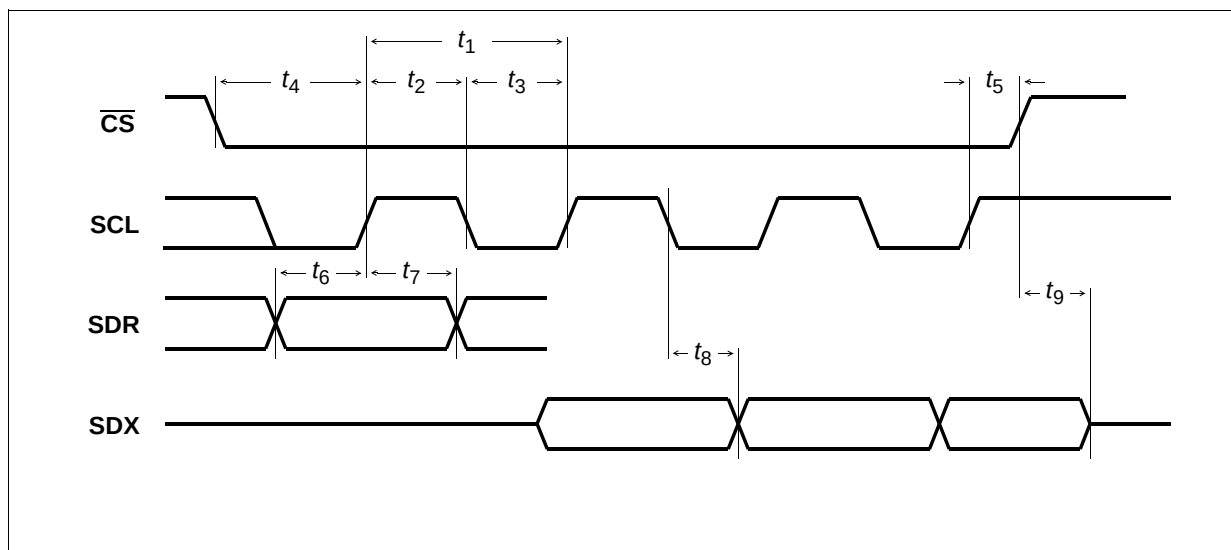
Figure 93 SCI Interface
