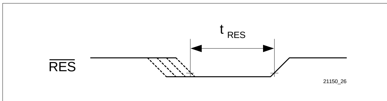
Figure 102 Reset Signal \overline{\text{RES}}
