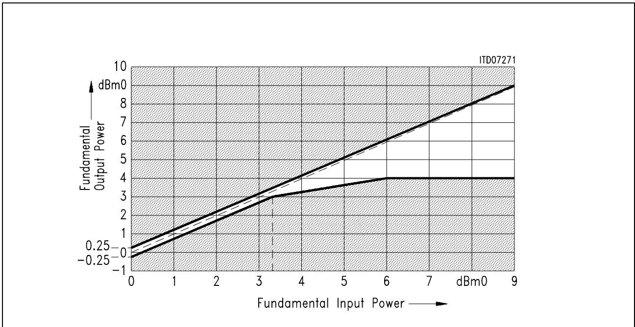
Figure 25 μ-Law, Transmit: measured with sine wave f = 1014 Hz.
