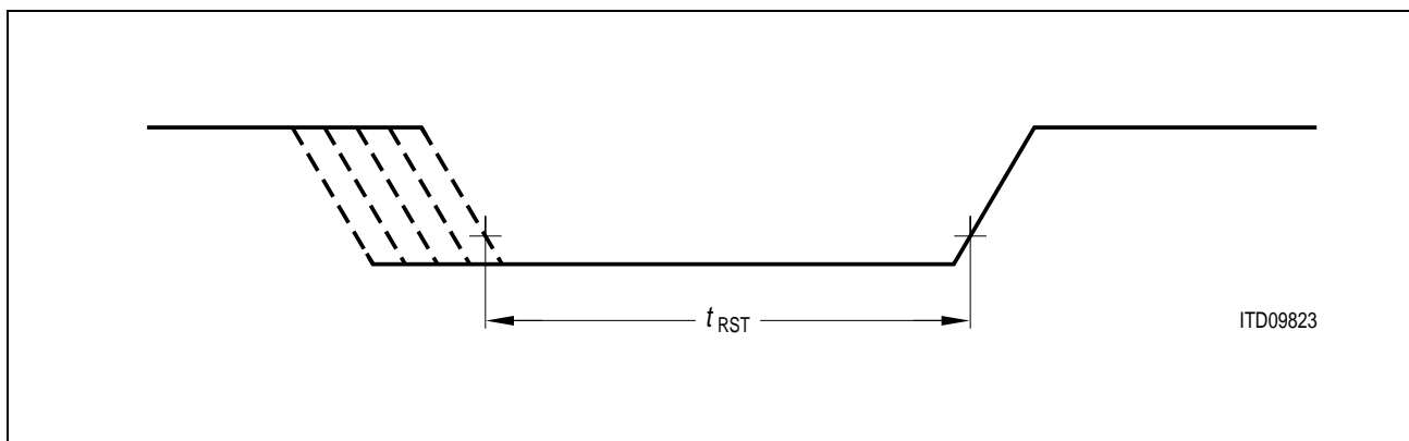
Figure 63 Reset Signal
