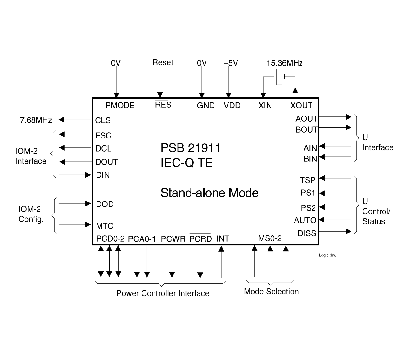
Figure 3 Logic Symbol Stand-Alone Mode
