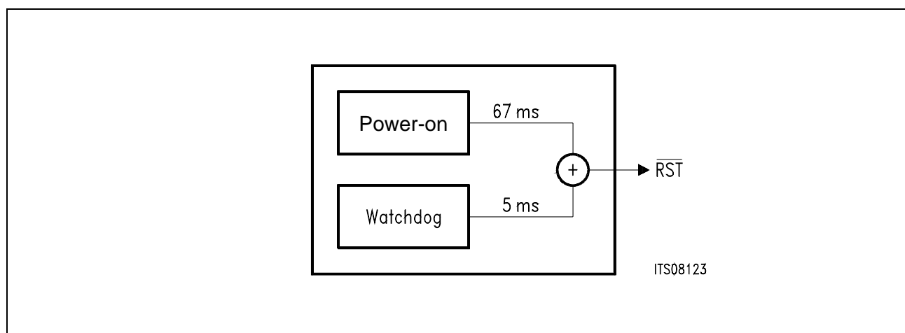
Figure 32 Reset Sources
