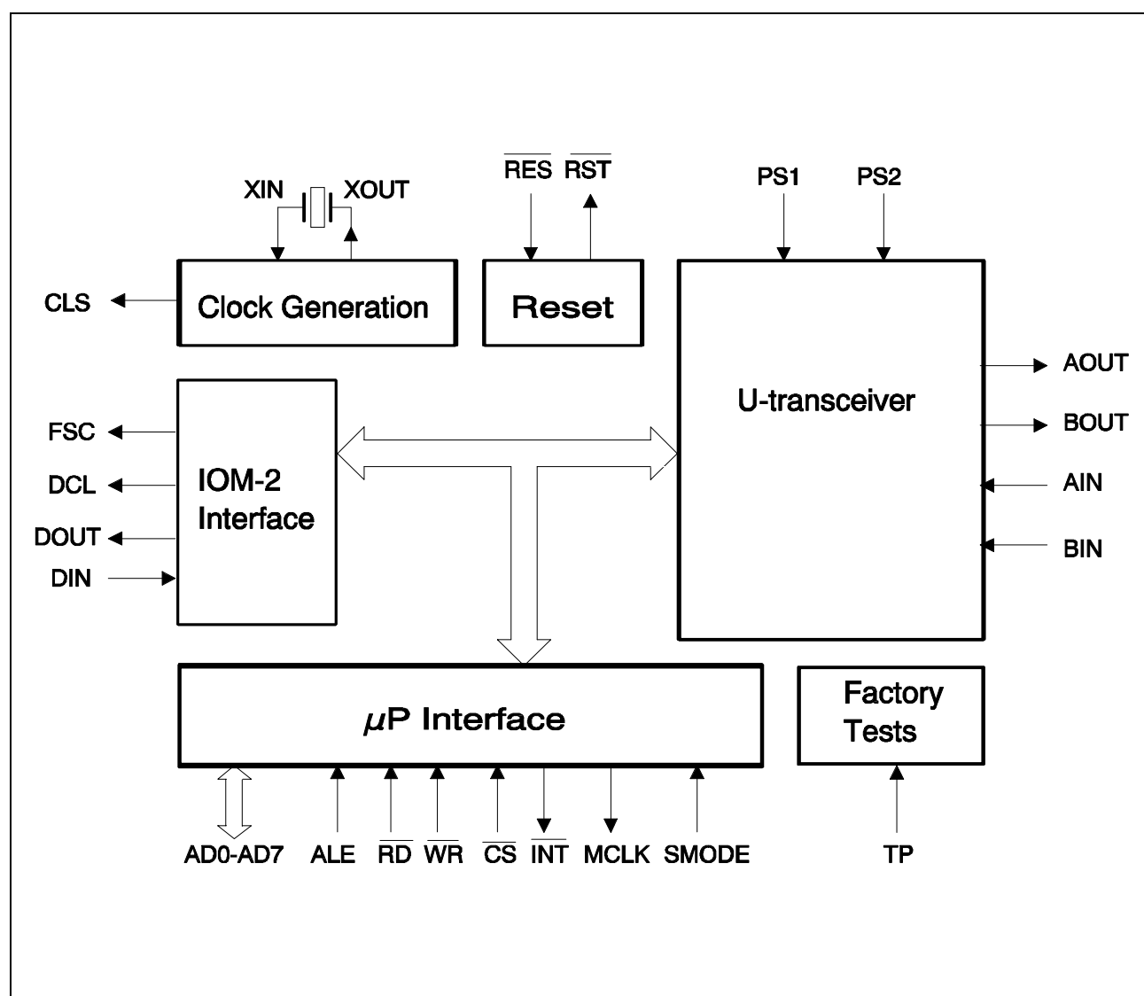
Figure 9 IEC-Q TE Device Architecture ( \mu P Mode)
