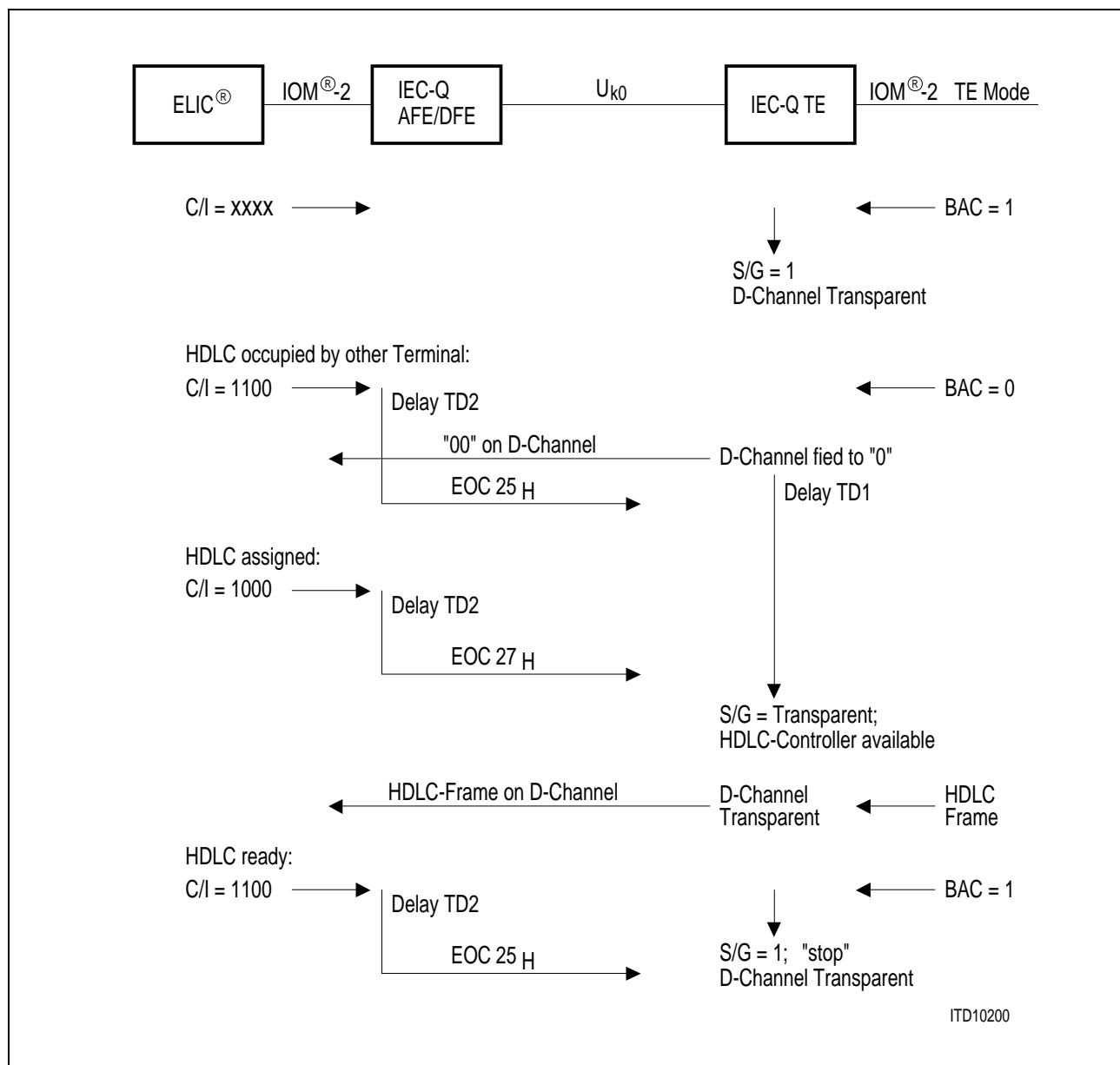
Figure 31 D-Channel Request by the Terminal
