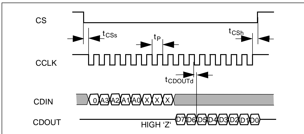
Figure 59 Serial μP Interface Mode Read
