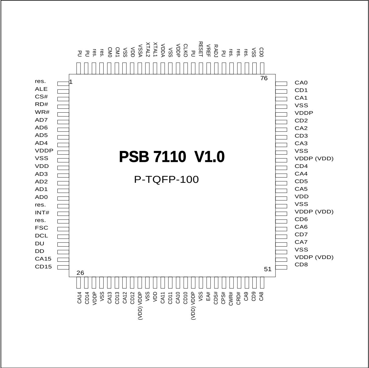
Figure 6 Pinout
