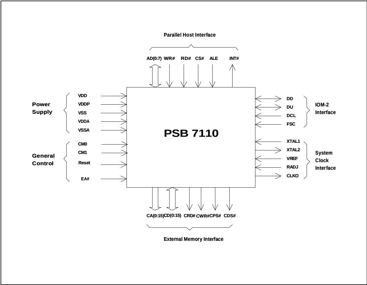
Figure 5 Logic symbol
