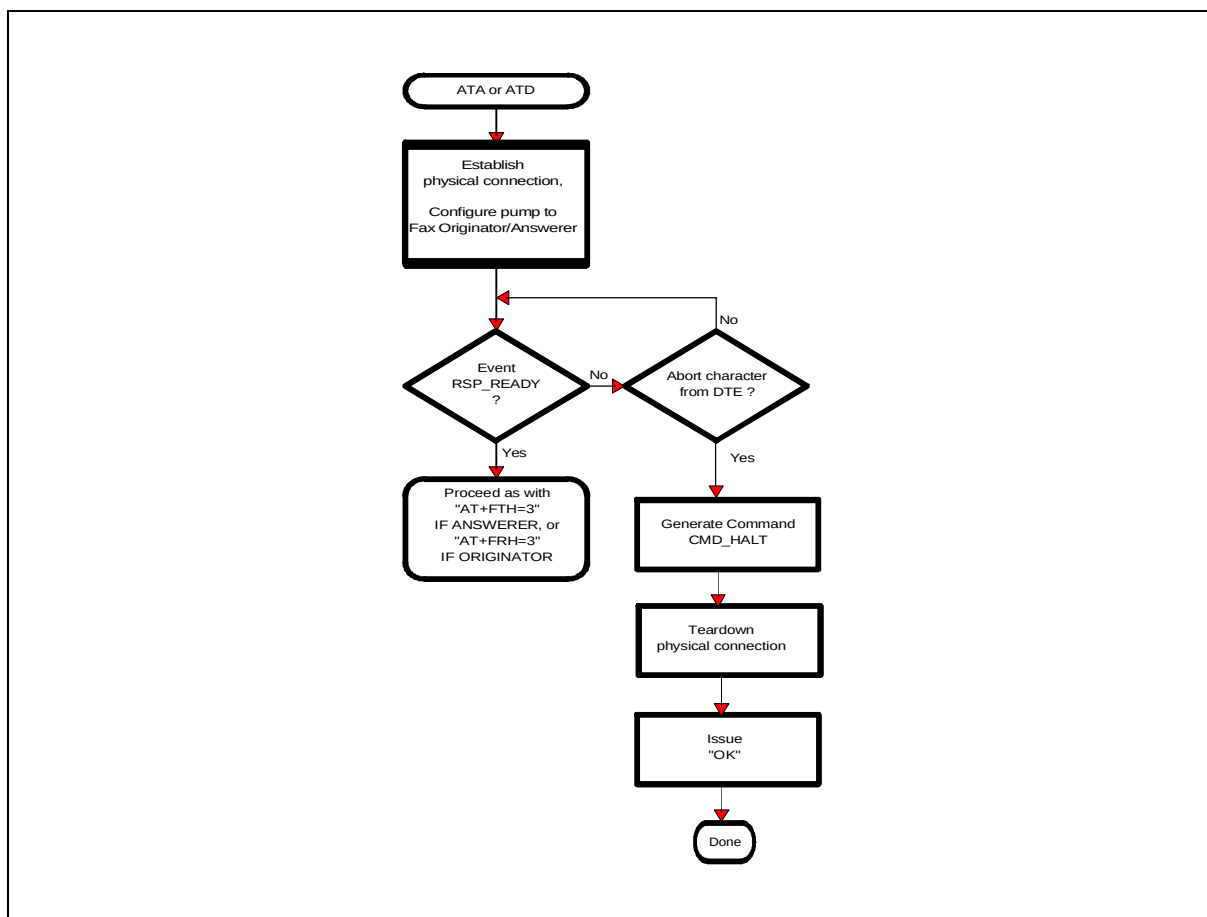
Figure 21 Startup procedure
