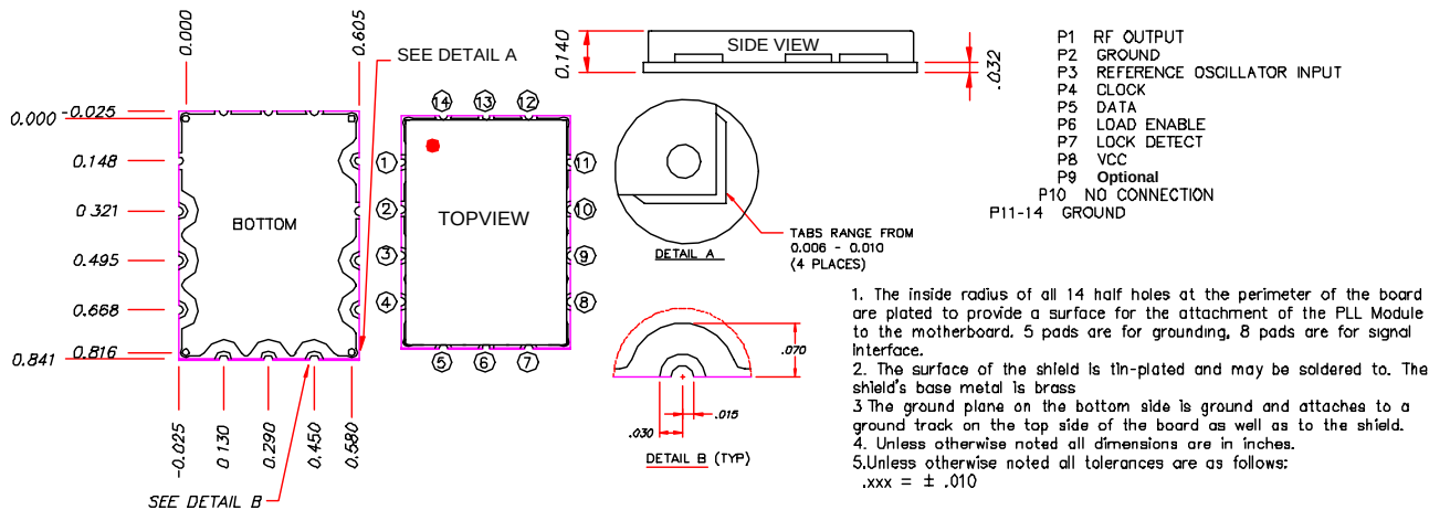
PHYSICAL DIMENSIONS
