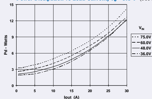
Power Dissipation vs Load Current; V_o = 3.3\text{ V} (See Note A)
