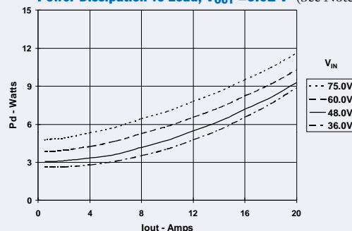
Power Dissipation vs Load; V_{OUT} = 5.02\text{ V} (See Note A)
