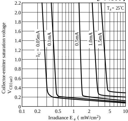
Fig. 9-a Collector-emitter Saturation Voltage vs. Irradiance
