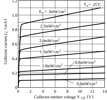
Fig. 5-d Collector Current vs. Collector-emitter Voltage (PT4810F)
