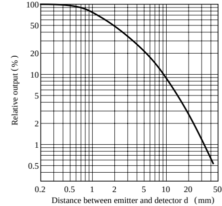
Fig.10-a Relative Output vs. Distance (PT4800F) (Emitter : GL4800)
