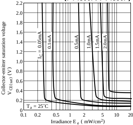
Fig. 9-b Collector-emitter Saturation Voltage vs. Irradiance
