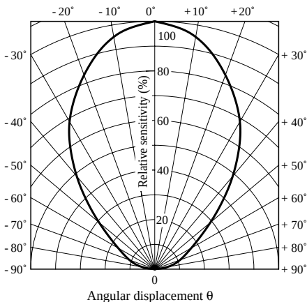
Fig. 8 Radiation Diagram ( T_a = 25^\circ\text{C} )
