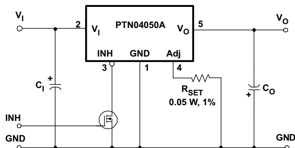
Figure 17. Inhibit Circuit
