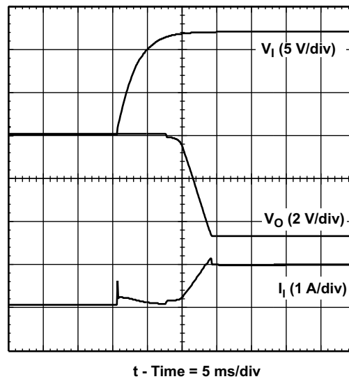
Figure 18. Power-Up Waveforms
