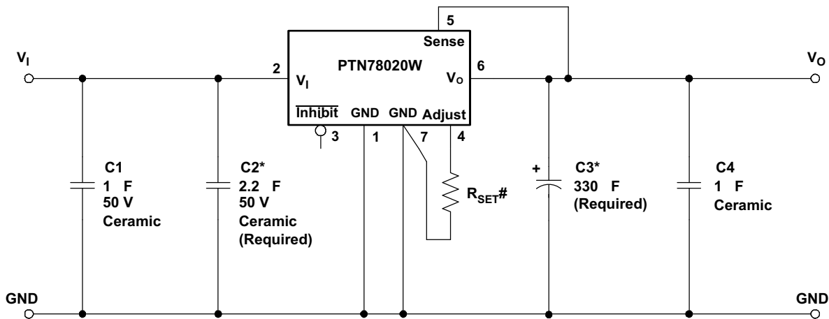
Figure 29. Adding High-Frequency Bypass Capacitors To The Input and Output
