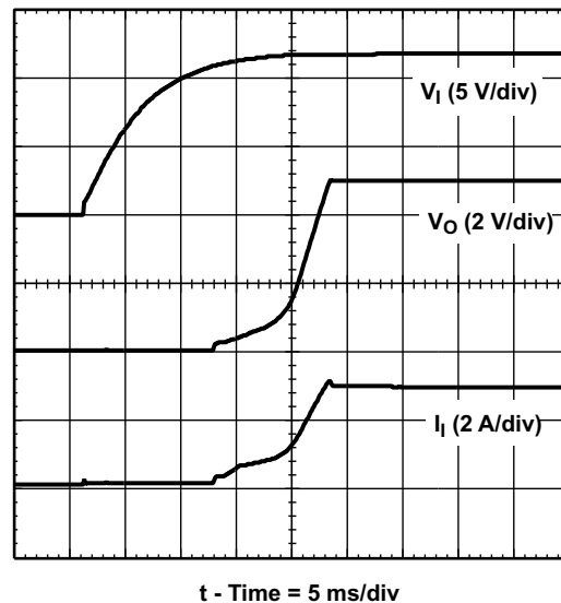
Figure 26. Power-Up Waveforms
