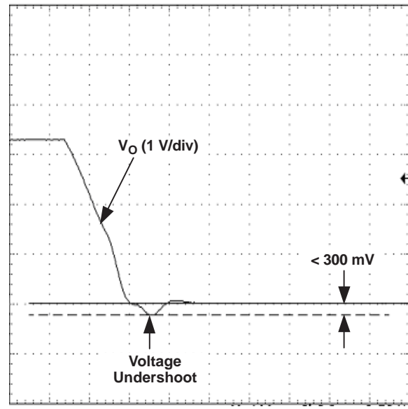
Figure 15. Power Down
