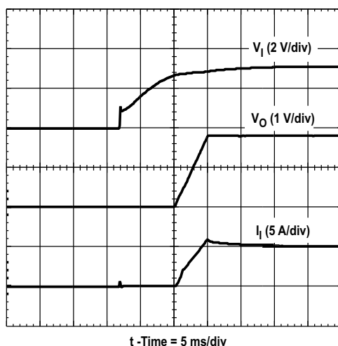
Figure 8. Power-Up Waveform
