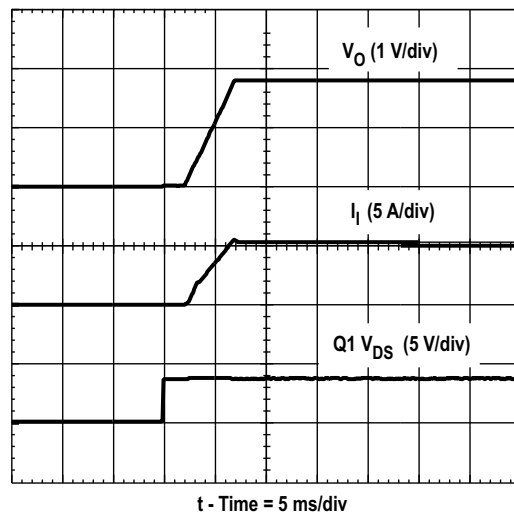
Figure 10. Inhibit Waveform
