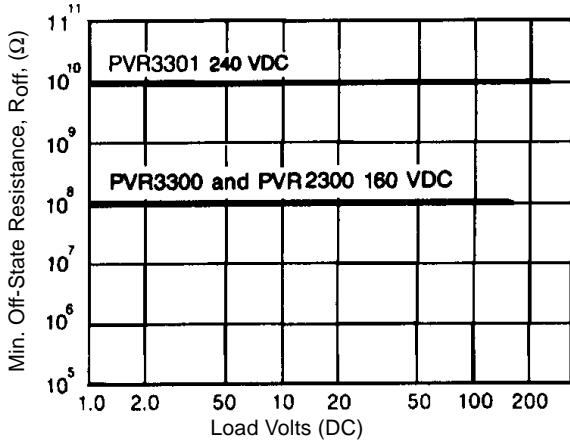
Figure 5. Off-State Resistance
