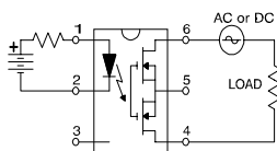
"A" Connection
