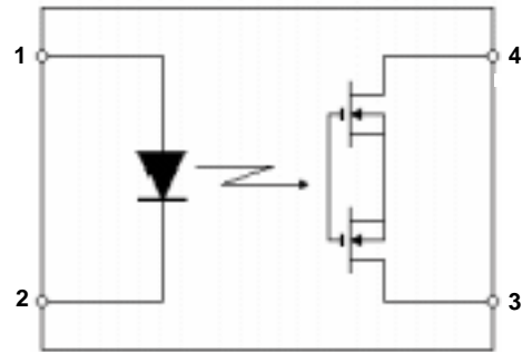
Connection Diagram
