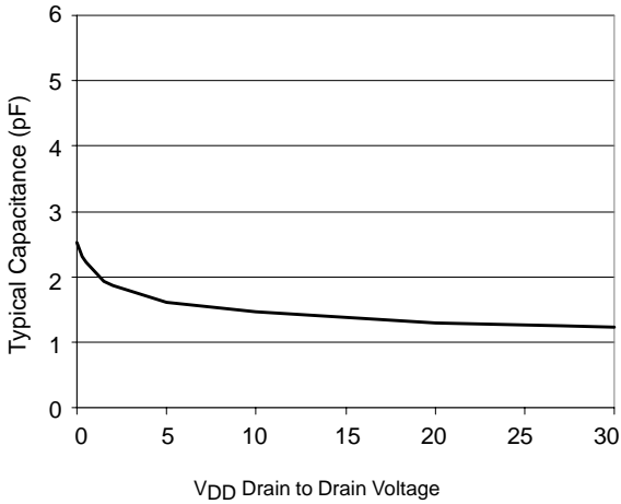
Figure 7. Output Capacitance
