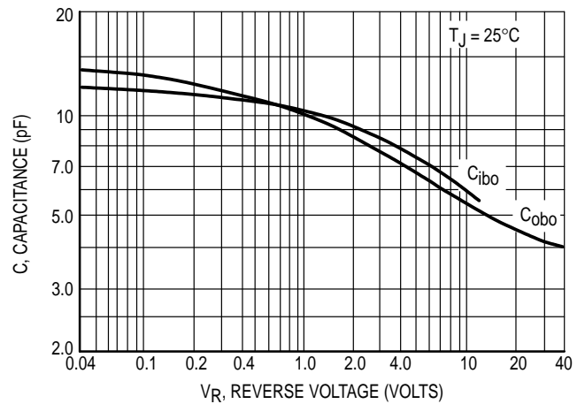
Figure 4. Capacitance
