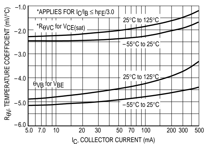
Figure 6. Temperature Coefficients
