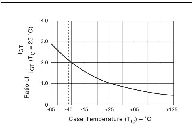
Figure E4.8 Normalized DC Gate Trigger Current for all Quadrants versus Case Temperature
