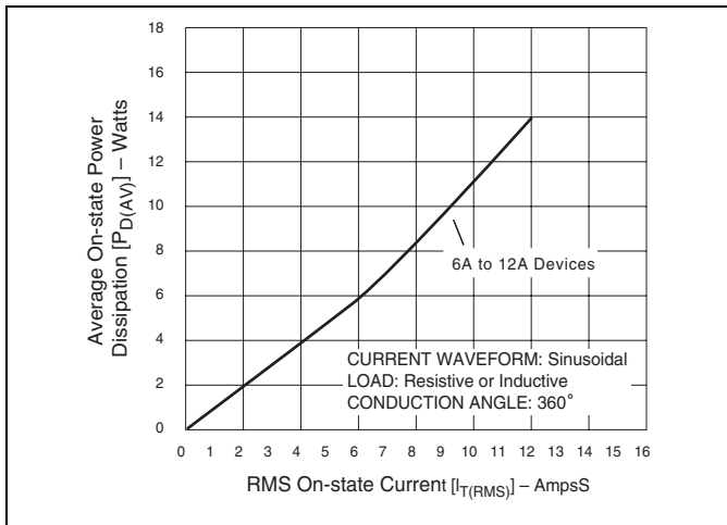
Figure E4.13 Power Dissipation (Typical) versus On-state Current (6 A to 12 A)
