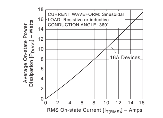
Figure E4.14 Power Dissipation (Typical) versus On-state Current (16 A)
