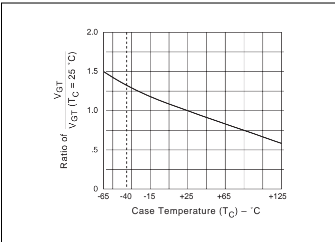
Figure E4.7 Normalized DC Gate Trigger Voltage for all Quadrants versus Case Temperature
