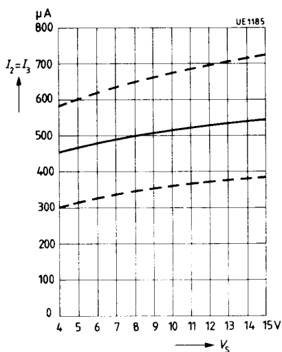
Output current versus supply voltage
