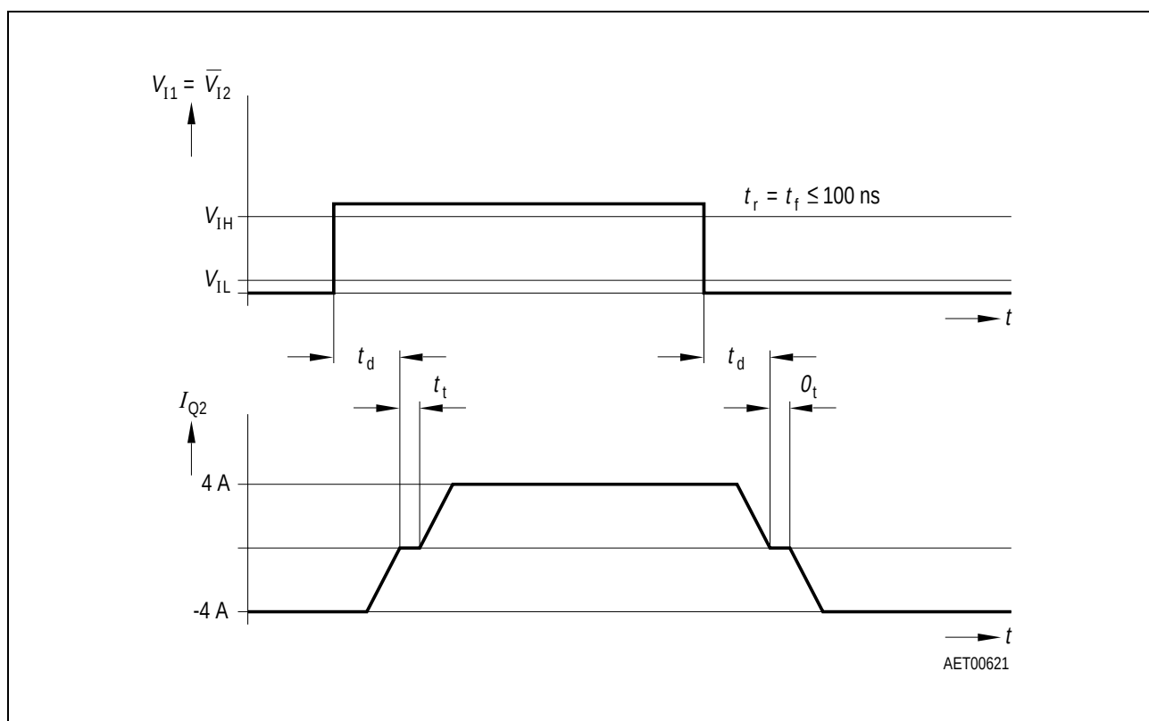
Figure 4 Timing Diagram
