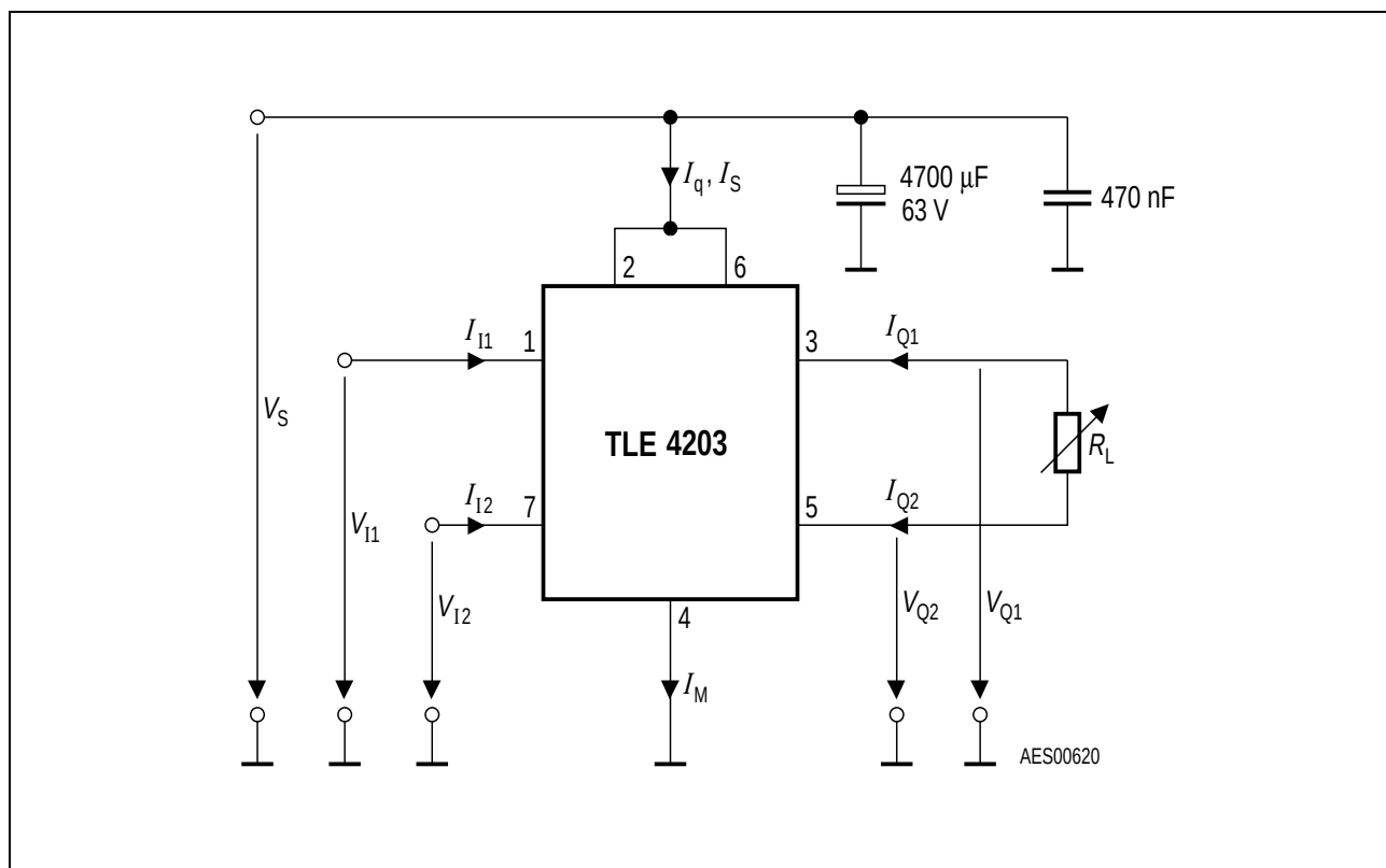
Figure 3 Test Circuit
