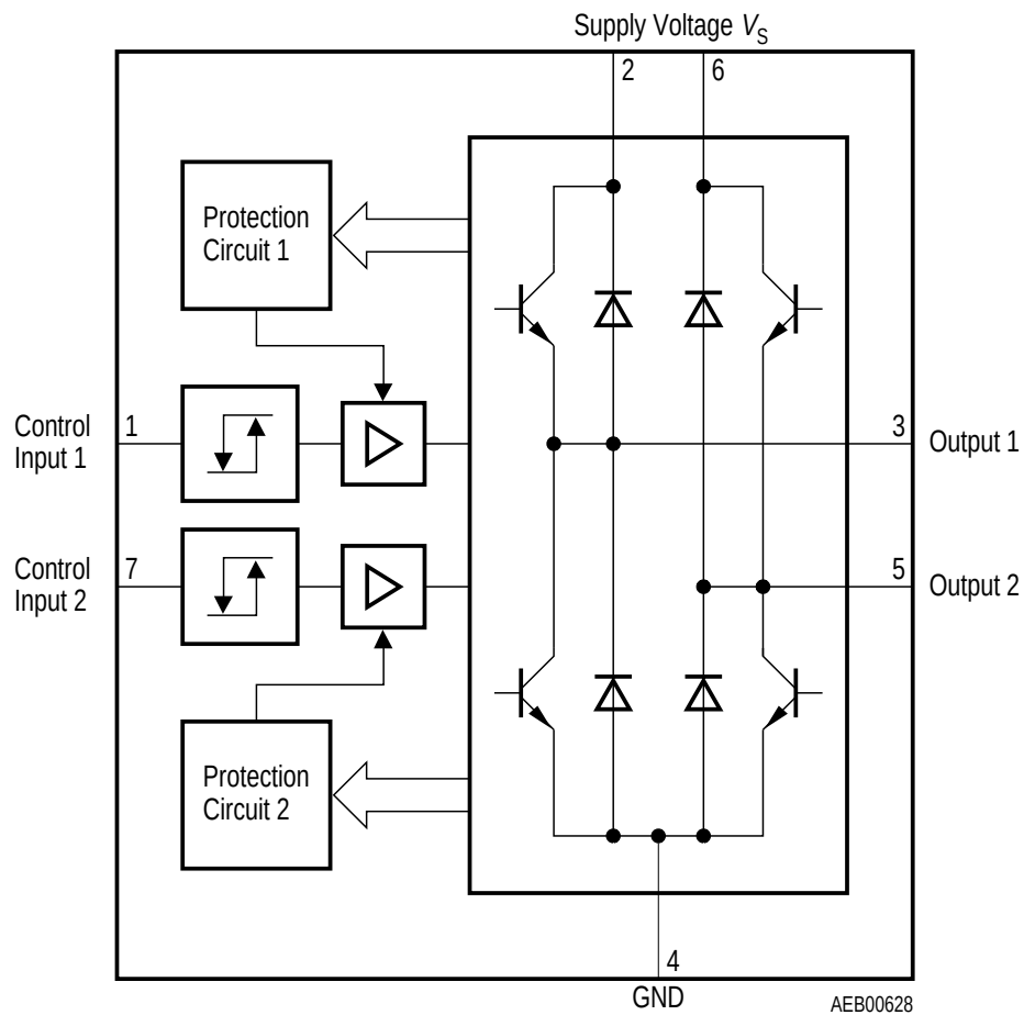
Figure 2 Block Diagram
