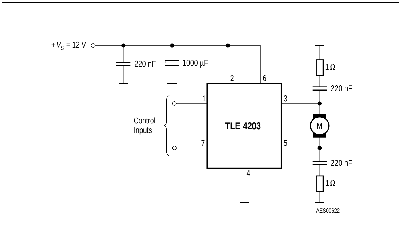
Figure 5 Application Circuit
