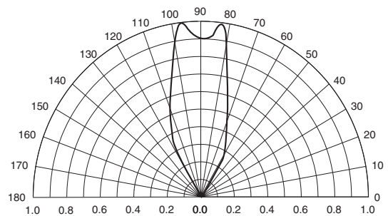
Fig. 4 Radiation Diagram
