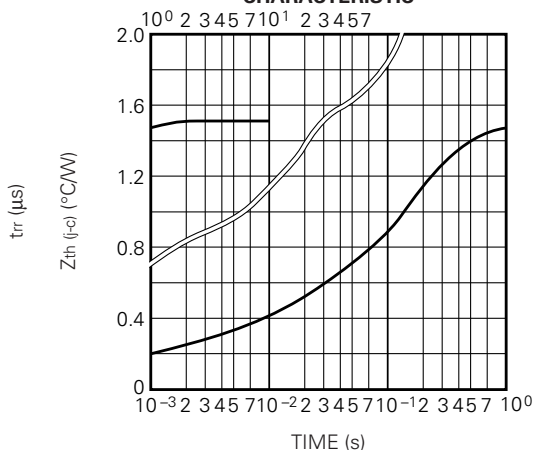
TRANSIENT THERMAL IMPEDANCE CHARACTERISTIC
