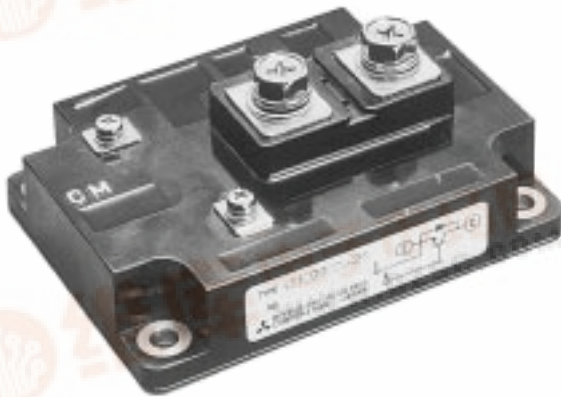
QM400HA-24
