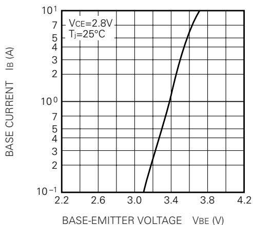
COMMON EMITTER INPUT CHARACTERISTIC (TYPICAL)
