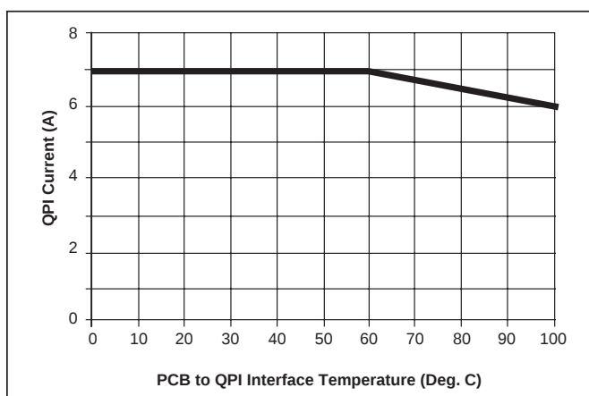
Figure 5 – QPI-3 current derating curve.
