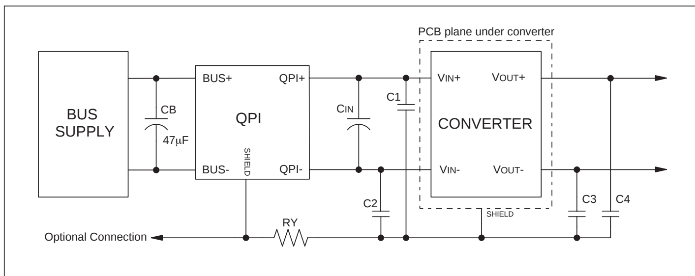
Figure 6 – Recommended schematic for QPI. Values of C_{IN} and C1 - C4 should be the values recommended by the converter manufacturer. If the manufacturer does not specify a value for the Y-capacitors use 4.7nF. R_Y=10\Omega , 1/4 W.
