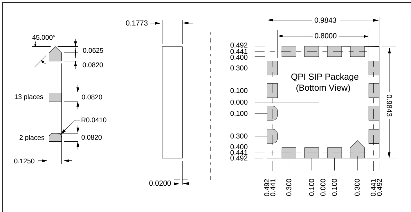
Figure 11 – QPI package dimensions and pad locations.
