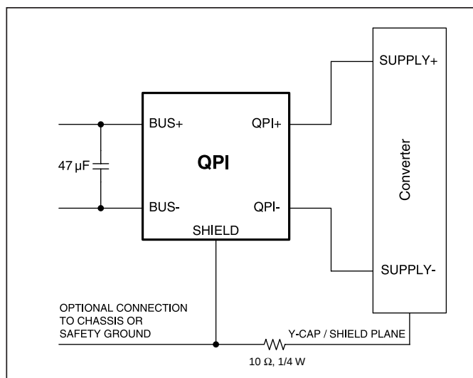
Figure 1 - QPI basic input bus filter circuit. Read important note on page 3 for Layout and Circuit Considerations.
