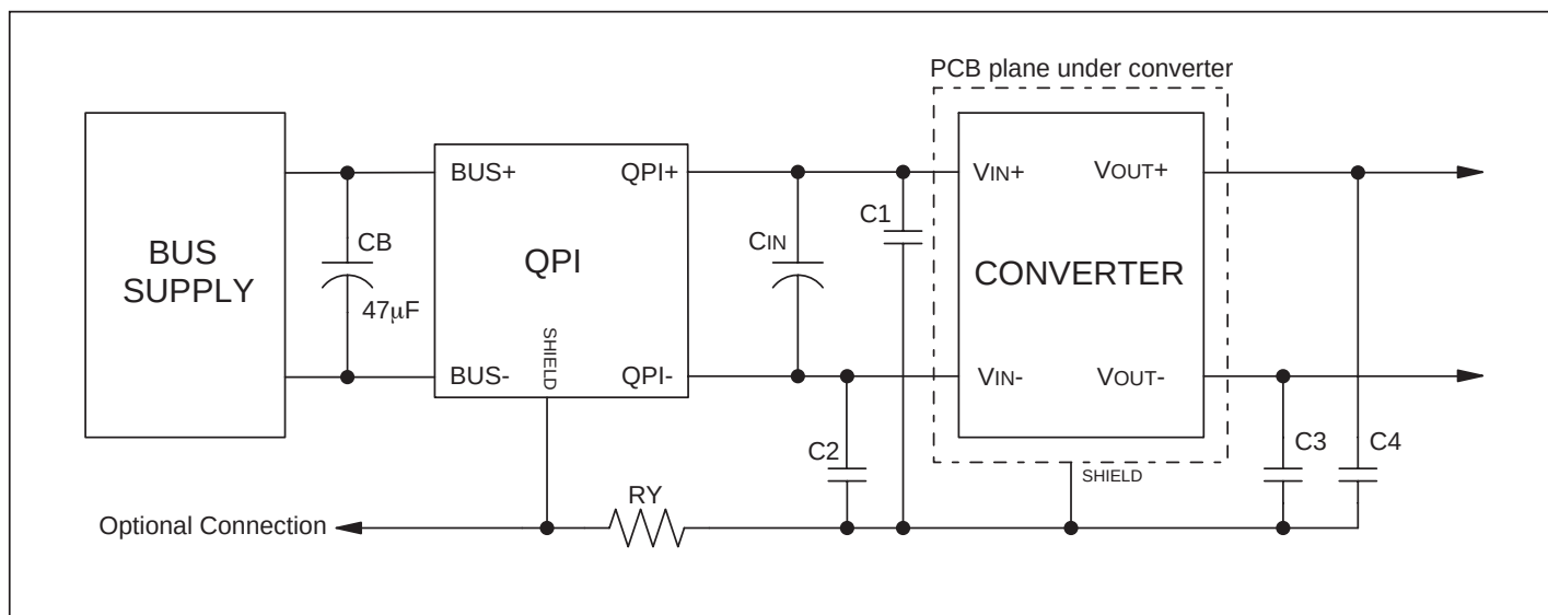
Figure 6 – Recommended schematic for QPI. Values of CIN and C1-C4 should be the values recommended by the converter manufacturer. If the manufacturer does not specify a value for the Y-capacitors use 4.7nF. Ry=10Ω, 1/4 W.
