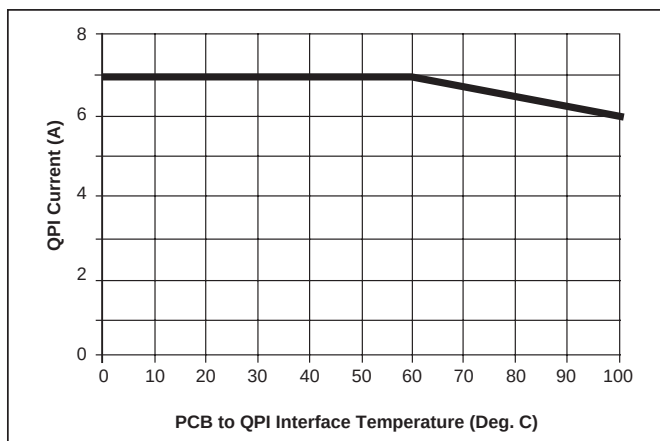
Figure 5 – QPI-4 current derating curve.
