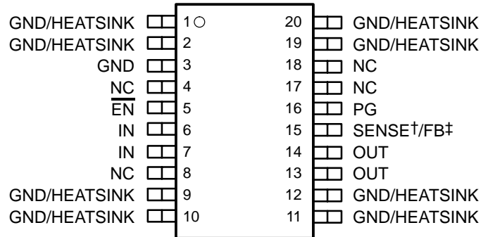
PWP PACKAGE (TOP VIEW)
