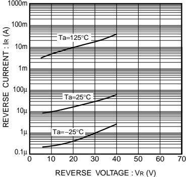
Fig.10 Reverse characteristics
