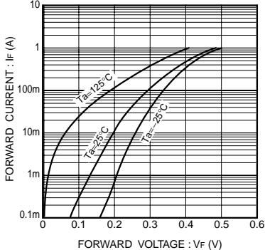
Fig.9 Forward characteristics
