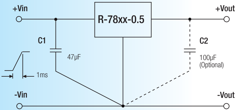
To protect the converter during power-up, use soft start Vin and C1=47µF
