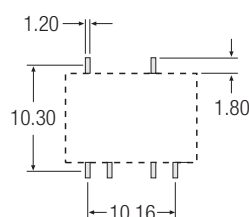
Recommended Footprint Details
