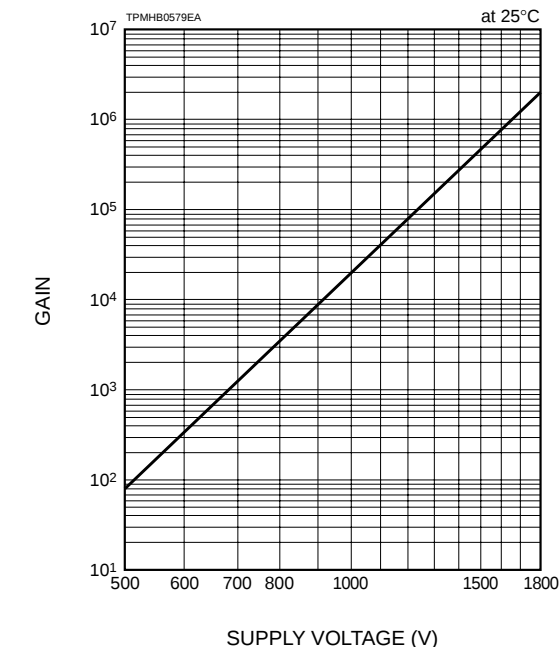
Figure 2: Typical Gain
