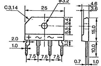
Outline Drawing 71
