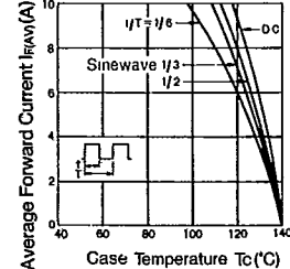
I F(AV) - T c Derating
