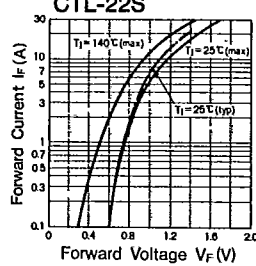
I F - V F Characteristics (Typical Value) CTL-22S
