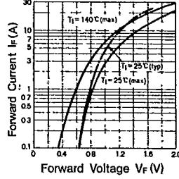
I F - V F Characteristics (Typical Value) CTL-22S
