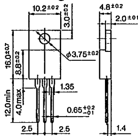
Outline Drawing 68
